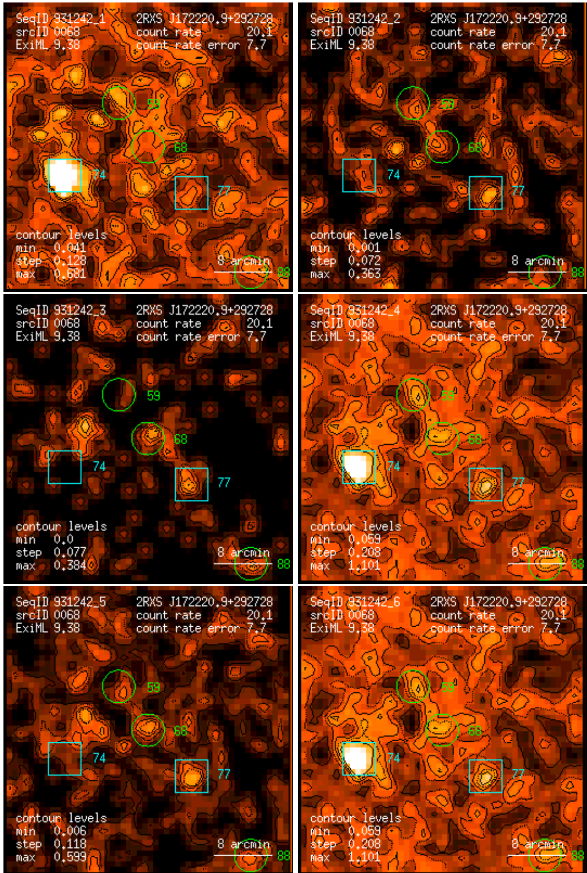
Figure 68: RASS 931242: detection 0068: band rate images, Gaussian filter: (1) PSPC channels 11 – 41, (2) 52 – 90, (3) 91 – 201, (4) 11 – 235, (5) 52 – 201, (6) 11 – 201. Broad band rates in counts/ks. Band rate contour levels in counts/ks/arcmin 2 .
