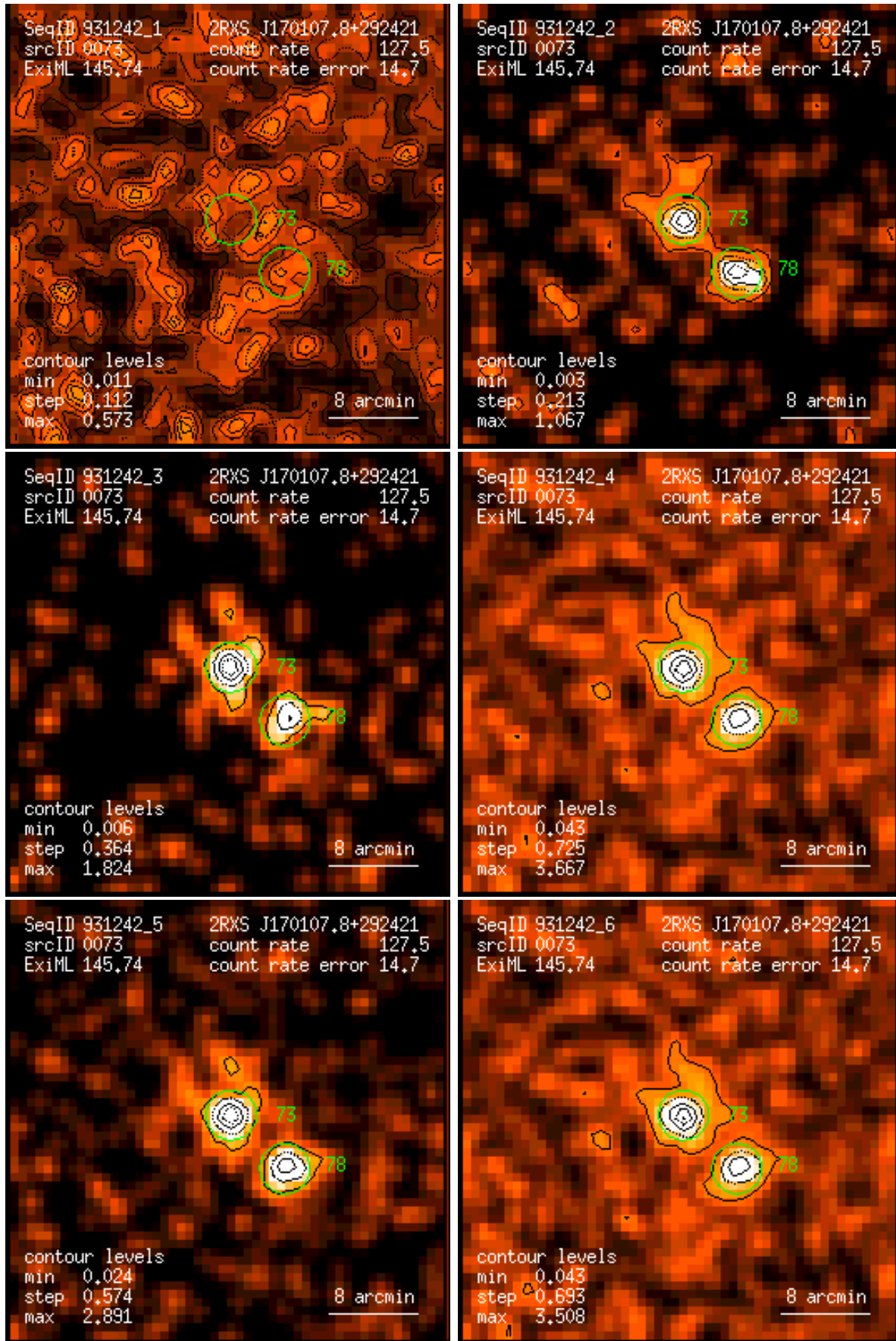
Figure 73: RASS 931242: detection 0073: band rate images, Gaussian filter: (1) PSPC channels 11 – 41, (2) 52 – 90, (3) 91 – 201, (4) 11 – 235, (5) 52 – 201, (6) 11 – 201. Broad band rates in counts/ks. Band rate contour levels in counts/ks/arcmin 2 .
