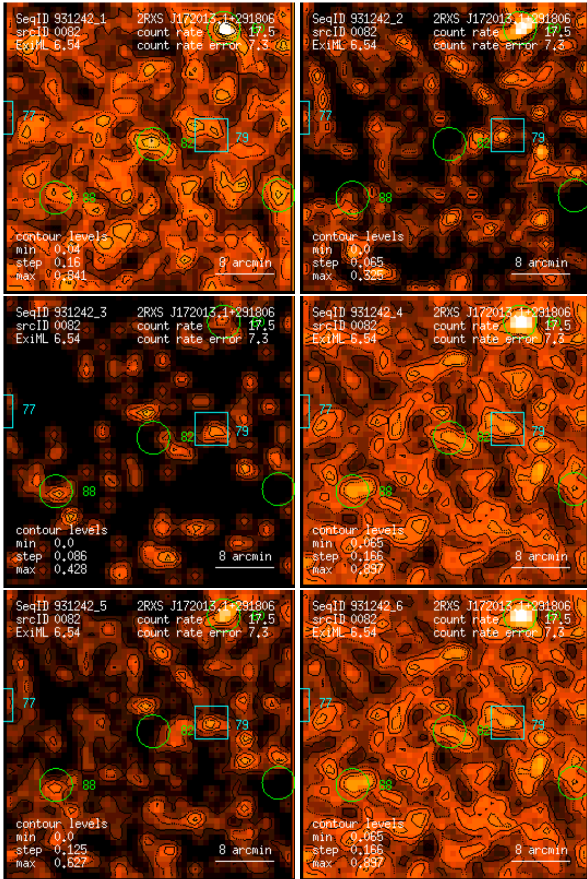
Figure 82: RASS 931242: detection 0082: band rate images, Gaussian filter: (1) PSPC channels 11 – 41, (2) 52 – 90, (3) 91 – 201, (4) 11 – 235, (5) 52 – 201, (6) 11 – 201. Broad band rates in counts/ks. Band rate contour levels in counts/ks/arcmin 2 .
