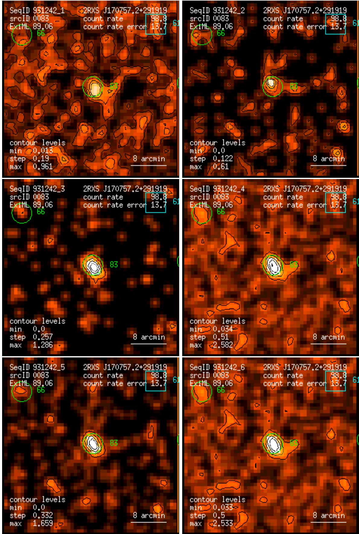
Figure 83: RASS 931242: detection 0083: band rate images, Gaussian filter: (1) PSPC channels 11 – 41, (2) 52 – 90, (3) 91 – 201, (4) 11 – 235, (5) 52 – 201, (6) 11 – 201. Broad band rates in counts/ks. Band rate contour levels in counts/ks/arcmin 2 .
