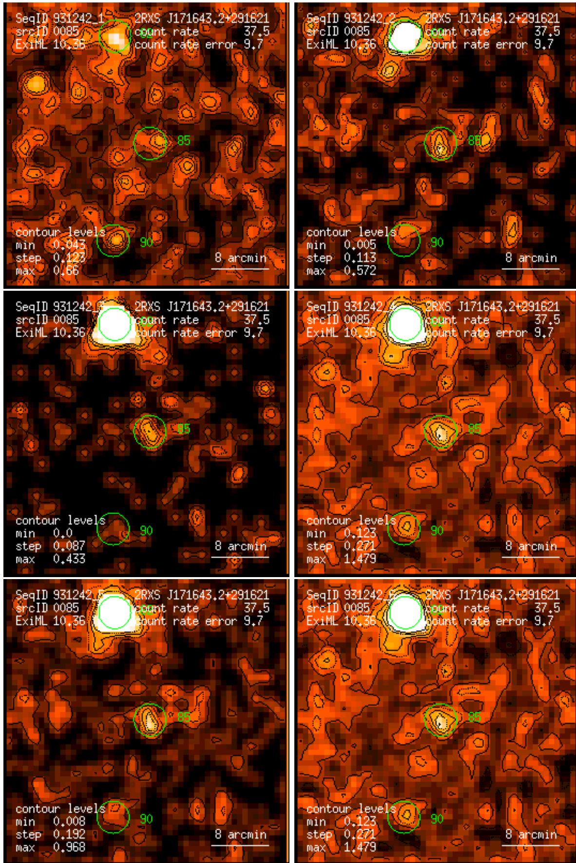
Figure 85: RASS 931242: detection 0085: band rate images, Gaussian filter: (1) PSPC channels 11 – 41, (2) 52 – 90, (3) 91 – 201, (4) 11 – 235, (5) 52 – 201, (6) 11 – 201. Broad band rates in counts/ks. Band rate contour levels in counts/ks/arcmin 2 .
