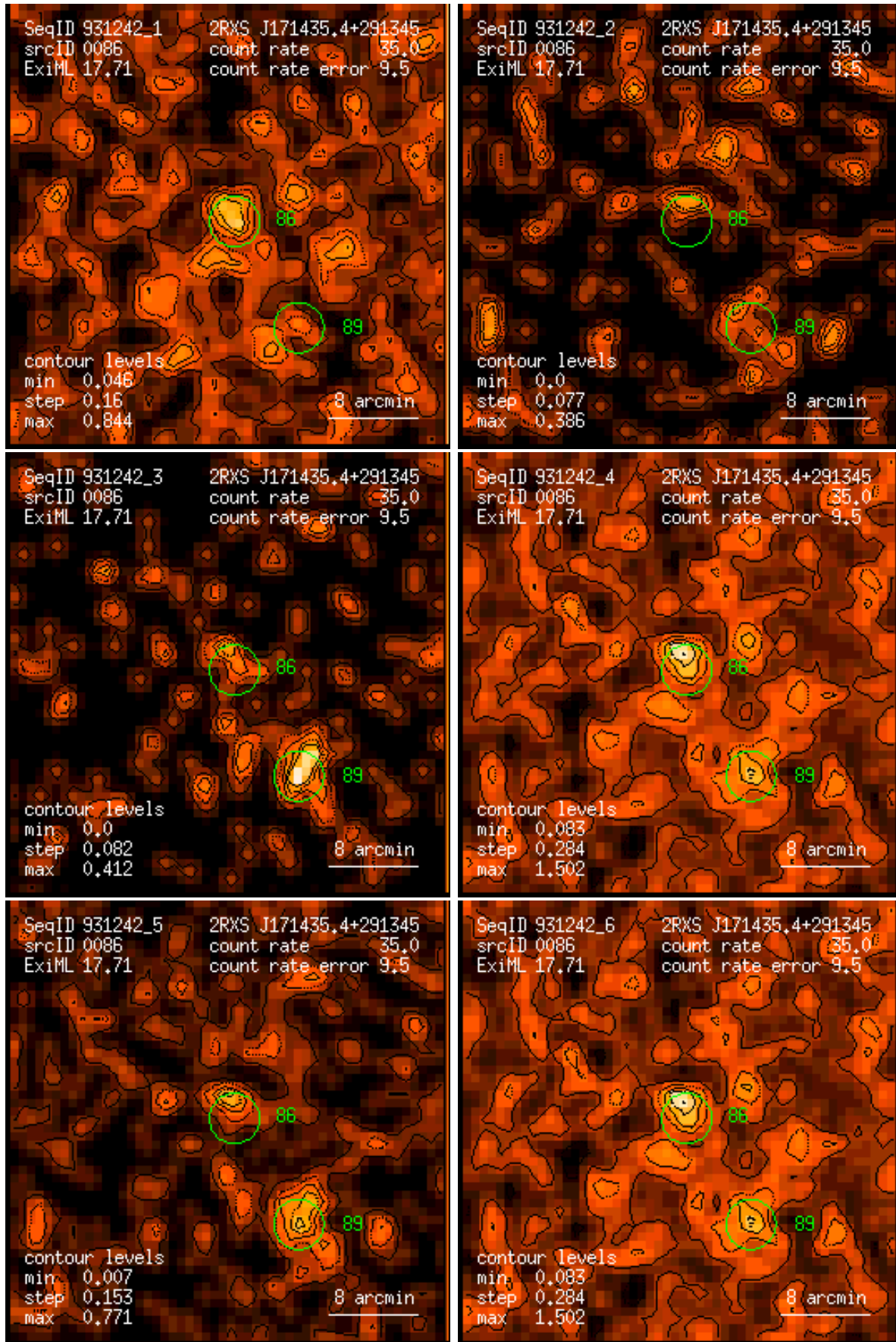
Figure 86: RASS 931242: detection 0086: band rate images, Gaussian filter: (1) PSPC channels 11 – 41, (2) 52 – 90, (3) 91 – 201, (4) 11 – 235, (5) 52 – 201, (6) 11 – 201. Broad band rates in counts/ks. Band rate contour levels in counts/ks/arcmin 2 .
