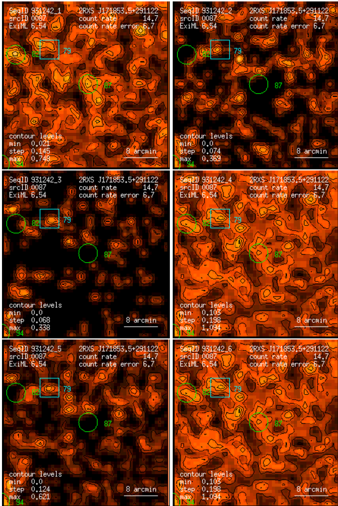
Figure 87: RASS 931242: detection 0087: band rate images, Gaussian filter: (1) PSPC channels 11 – 41, (2) 52 – 90, (3) 91 – 201, (4) 11 – 235, (5) 52 – 201, (6) 11 – 201. Broad band rates in counts/ks. Band rate contour levels in counts/ks/arcmin 2 .
