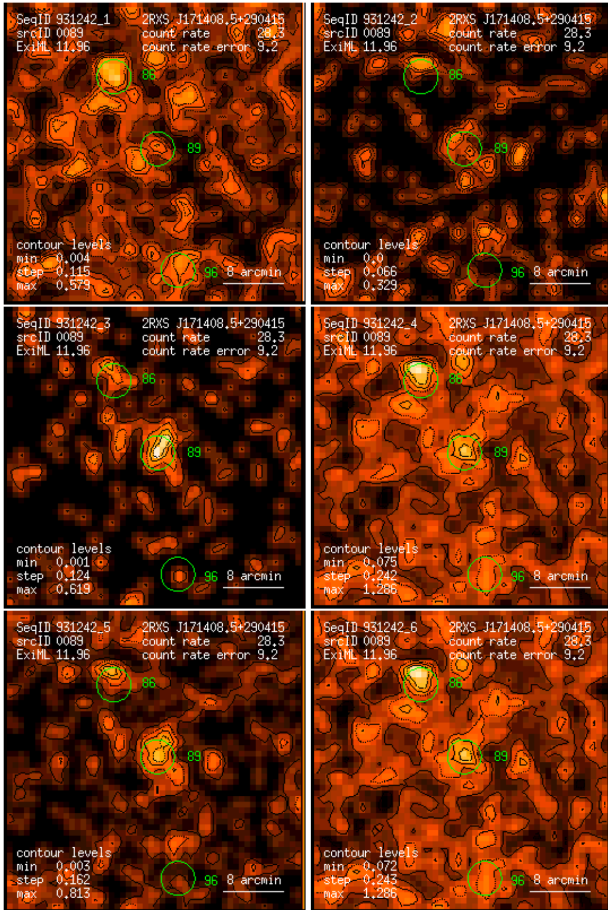
Figure 89: RASS 931242: detection 0089: band rate images, Gaussian filter: (1) PSPC channels 11 – 41, (2) 52 – 90, (3) 91 – 201, (4) 11 – 235, (5) 52 – 201, (6) 11 – 201. Broad band rates in counts/ks. Band rate contour levels in counts/ks/arcmin 2 .
