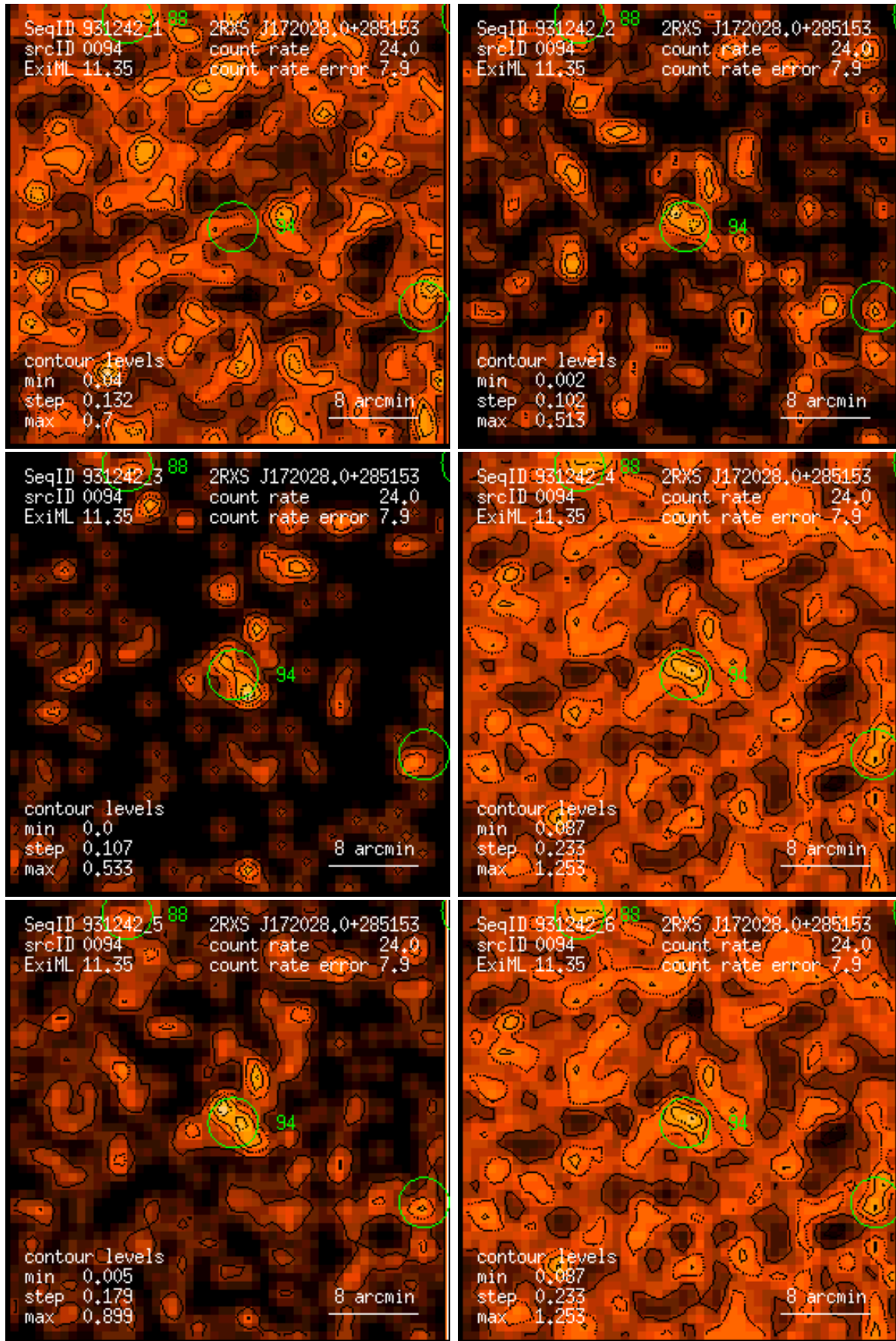
Figure 94: RASS 931242: detection 0094: band rate images, Gaussian filter: (1) PSPC channels 11 – 41, (2) 52 – 90, (3) 91 – 201, (4) 11 – 235, (5) 52 – 201, (6) 11 – 201. Broad band rates in counts/ks. Band rate contour levels in counts/ks/arcmin 2 .
