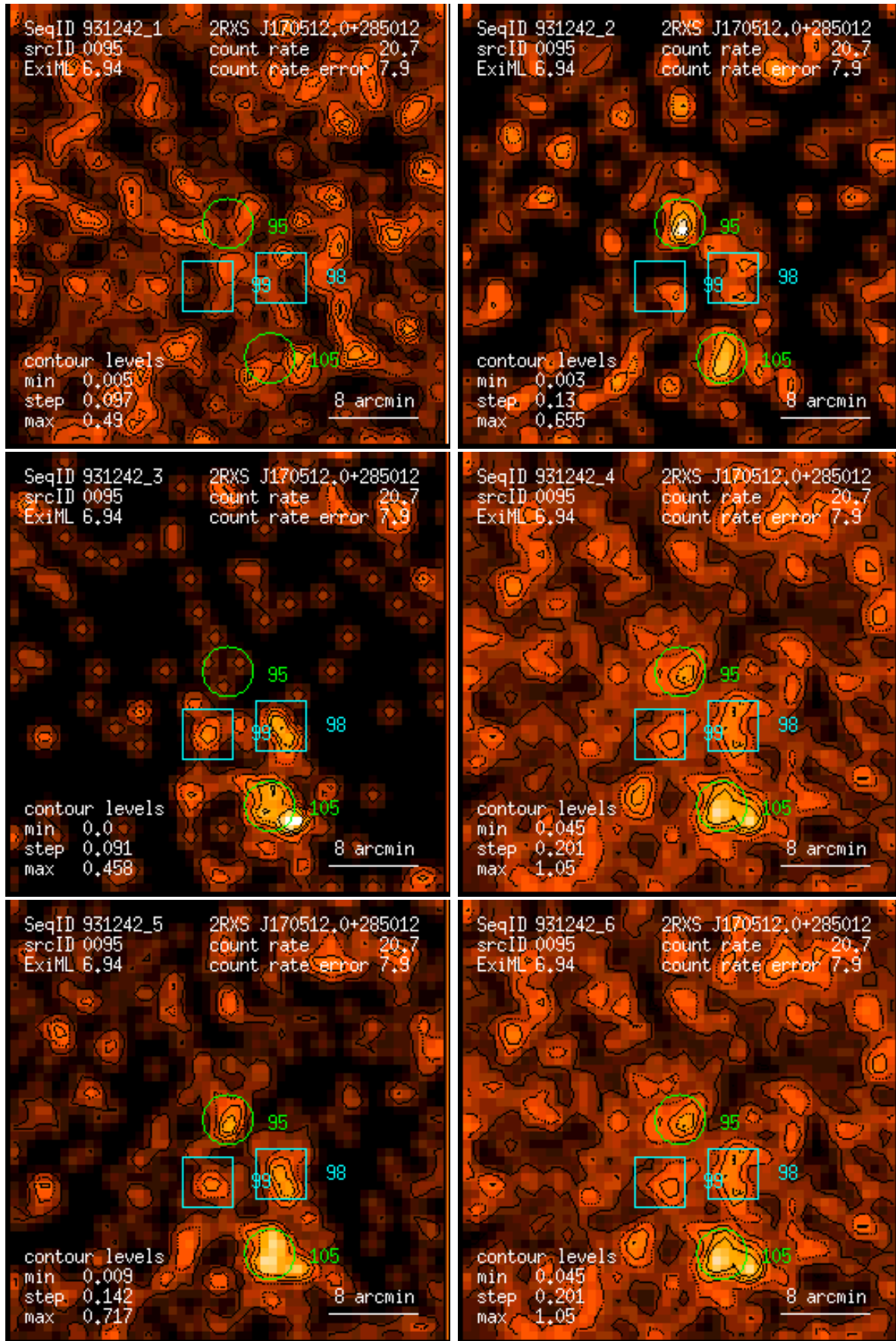
Figure 95: RASS 931242: detection 0095: band rate images, Gaussian filter: (1) PSPC channels 11 – 41, (2) 52 – 90, (3) 91 – 201, (4) 11 – 235, (5) 52 – 201, (6) 11 – 201. Broad band rates in counts/ks. Band rate contour levels in counts/ks/arcmin 2 .
