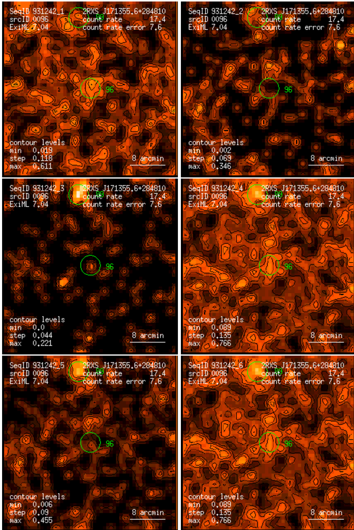
Figure 96: RASS 931242: detection 0096: band rate images, Gaussian filter: (1) PSPC channels 11 – 41, (2) 52 – 90, (3) 91 – 201, (4) 11 – 235, (5) 52 – 201, (6) 11 – 201. Broad band rates in counts/ks. Band rate contour levels in counts/ks/arcmin 2 .
