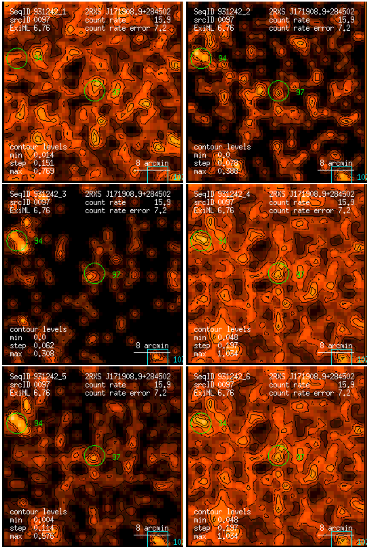
Figure 97: RASS 931242: detection 0097: band rate images, Gaussian filter: (1) PSPC channels 11 – 41, (2) 52 – 90, (3) 91 – 201, (4) 11 – 235, (5) 52 – 201, (6) 11 – 201. Broad band rates in counts/ks. Band rate contour levels in counts/ks/arcmin 2 .
