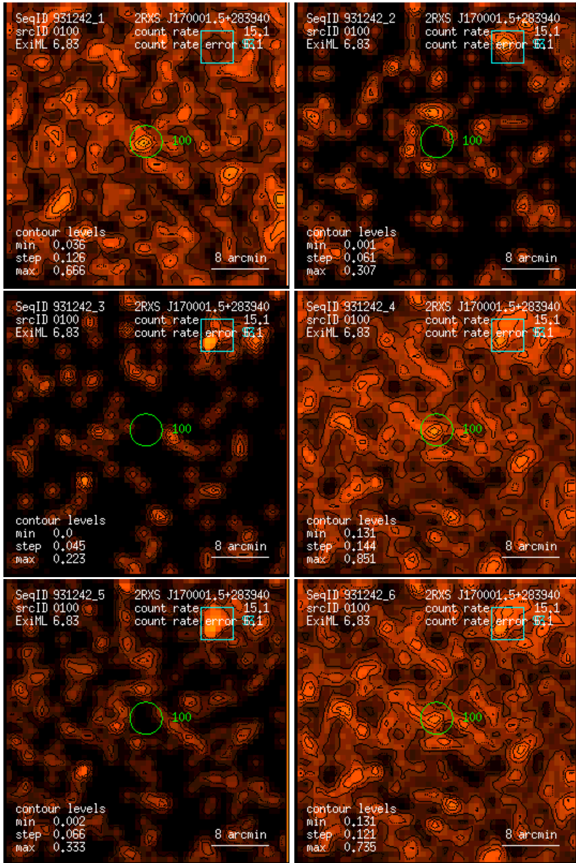
Figure 100: RASS 931242: detection 0100: band rate images, Gaussian filter: (1) PSPC channels 11 – 41, (2) 52 – 90, (3) 91 – 201, (4) 11 – 235, (5) 52 – 201, (6) 11 – 201. Broad band rates in counts/ks. Band rate contour levels in counts/ks/arcmin 2 .
