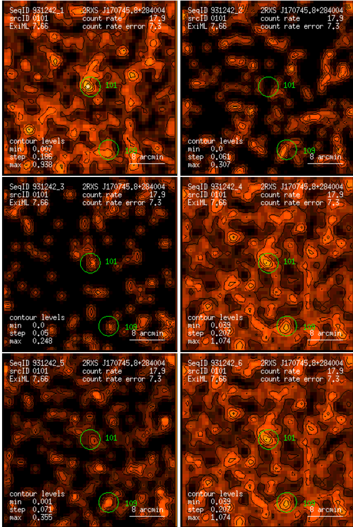
Figure 101: RASS 931242: detection 0101: band rate images, Gaussian filter: (1) PSPC channels 11 – 41, (2) 52 – 90, (3) 91 – 201, (4) 11 – 235, (5) 52 – 201, (6) 11 – 201. Broad band rates in counts/ks. Band rate contour levels in counts/ks/arcmin 2 .
