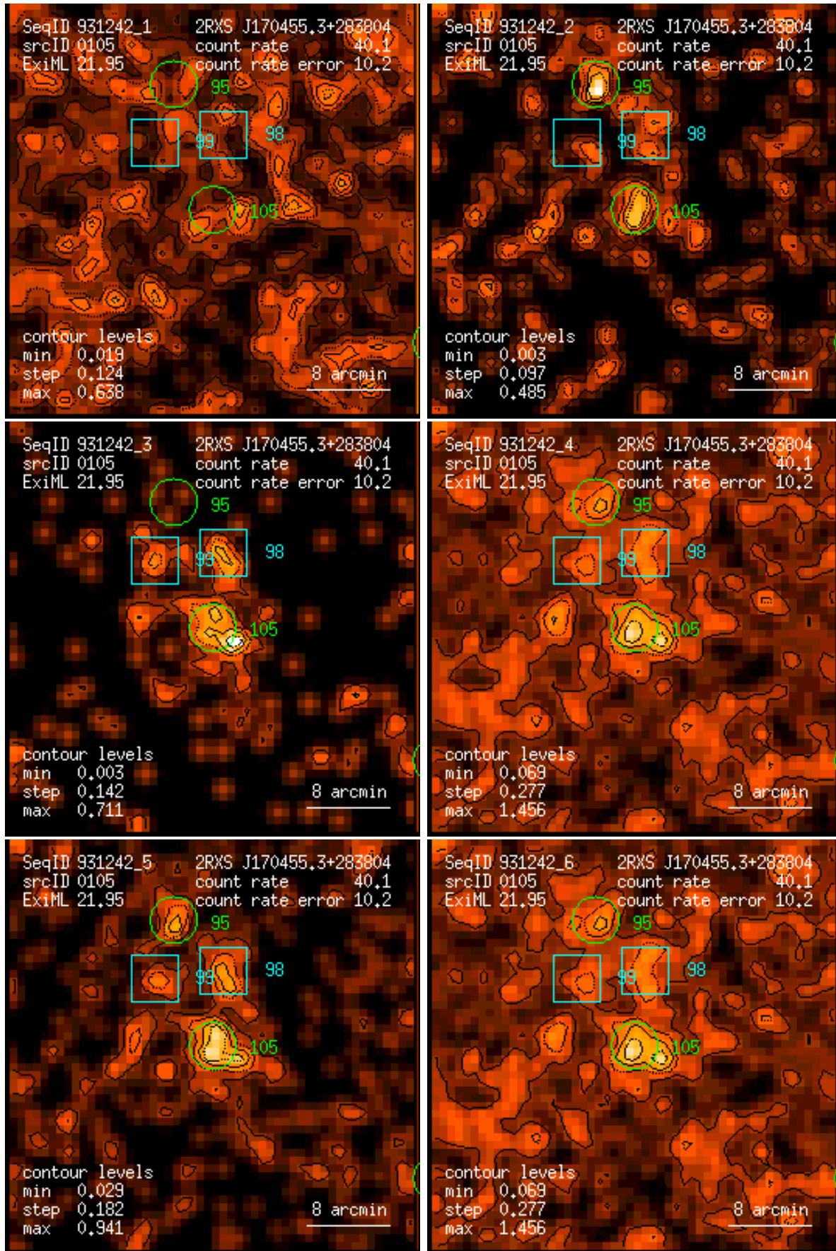
Figure 105: RASS 931242: detection 0105: band rate images, Gaussian filter: (1) PSPC channels 11 – 41, (2) 52 – 90, (3) 91 – 201, (4) 11 – 235, (5) 52 – 201, (6) 11 – 201. Broad band rates in counts/ks. Band rate contour levels in counts/ks/arcmin 2 .
