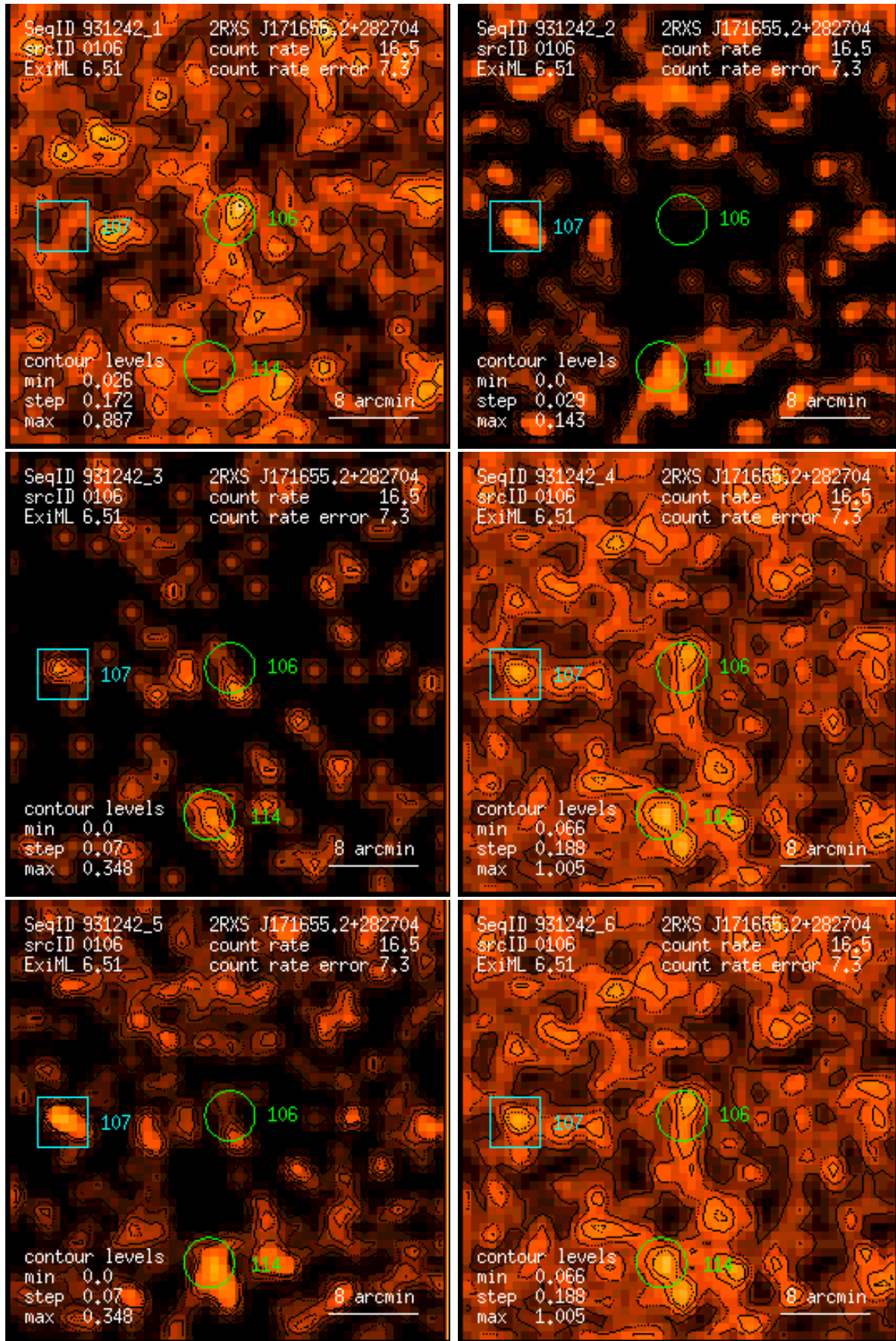
Figure 106: RASS 931242: detection 0106: band rate images, Gaussian filter: (1) PSPC channels 11 – 41, (2) 52 – 90, (3) 91 – 201, (4) 11 – 235, (5) 52 – 201, (6) 11 – 201. Broad band rates in counts/ks. Band rate contour levels in counts/ks/arcmin 2 .
