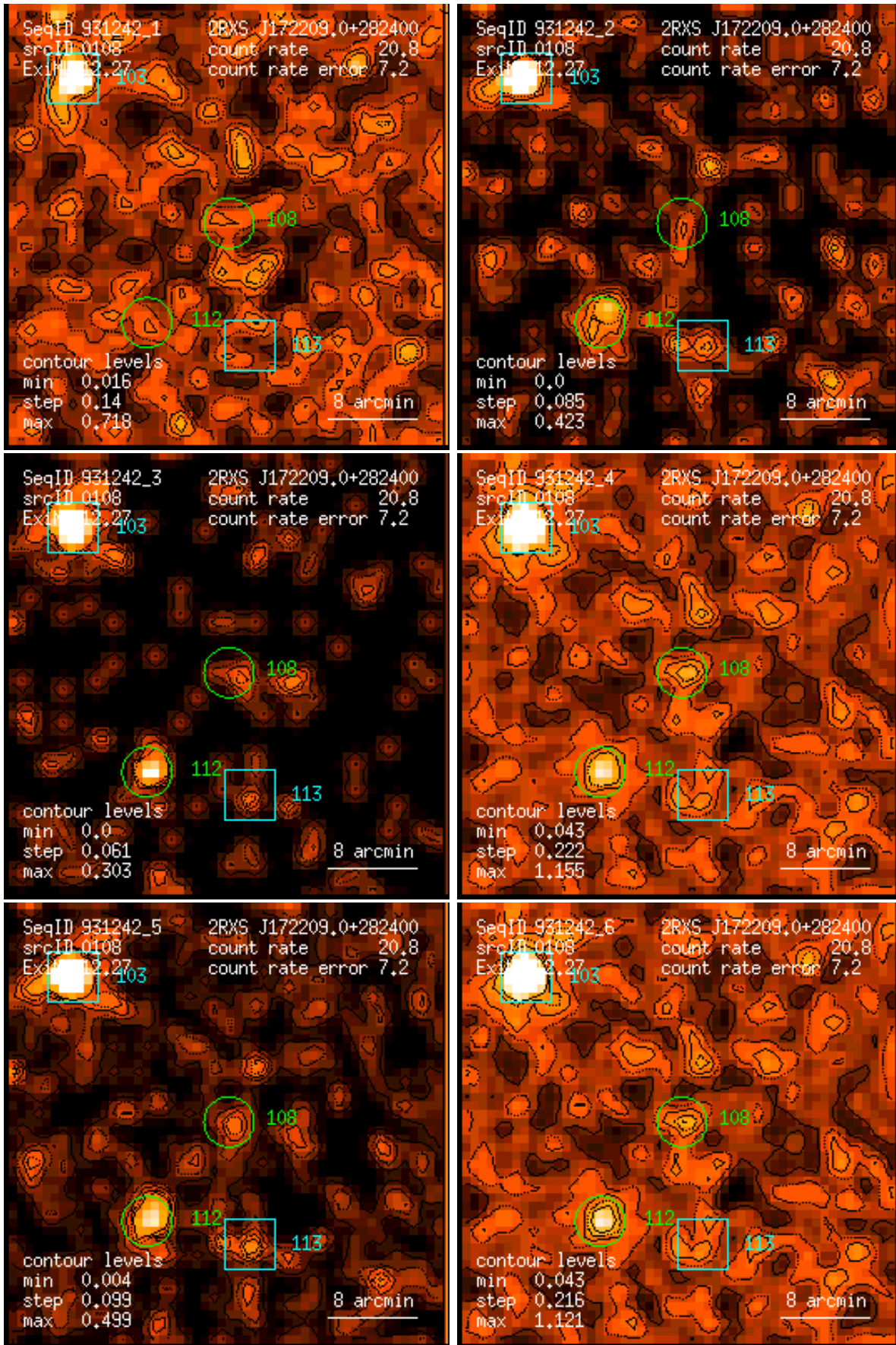
Figure 108: RASS 931242: detection 0108: band rate images, Gaussian filter: (1) PSPC channels 11 – 41, (2) 52 – 90, (3) 91 – 201, (4) 11 – 235, (5) 52 – 201, (6) 11 – 201. Broad band rates in counts/ks. Band rate contour levels in counts/ks/arcmin 2 .
