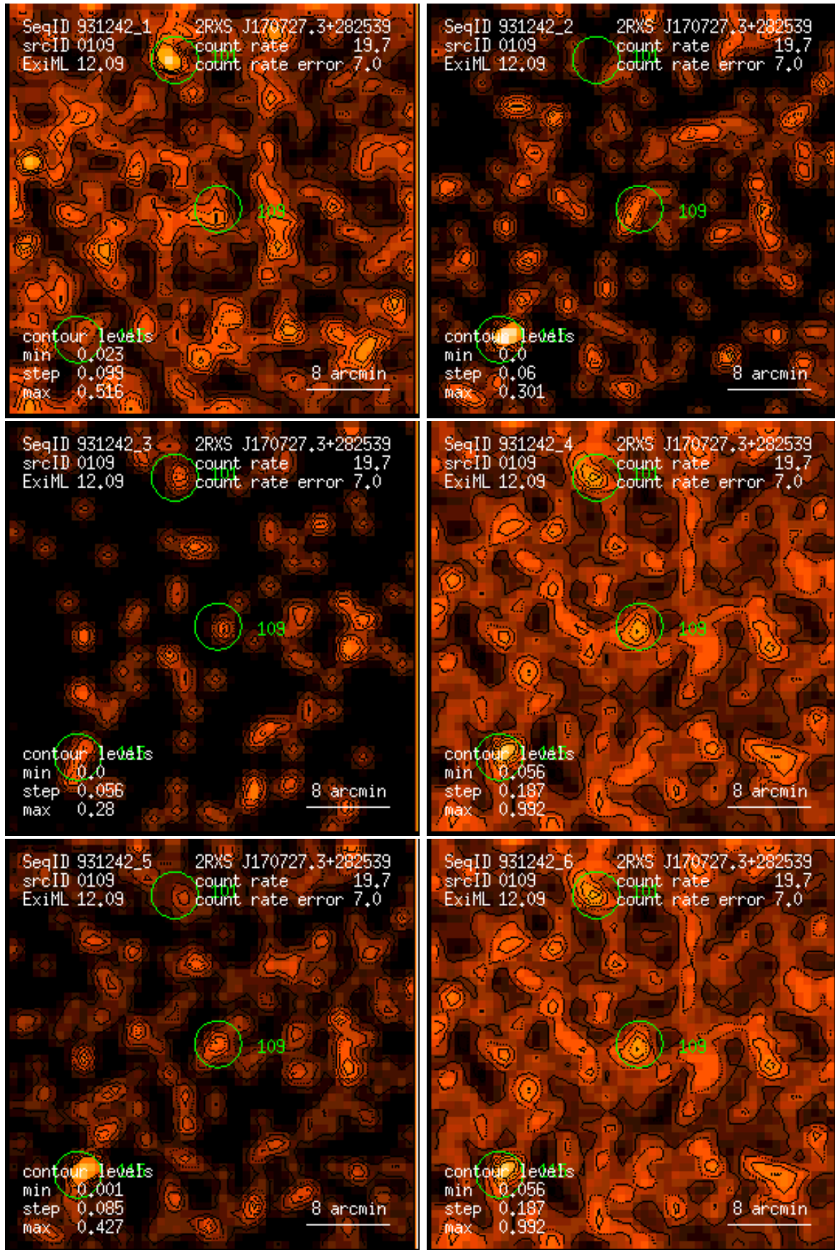
Figure 109: RASS 931242: detection 0109: band rate images, Gaussian filter: (1) PSPC channels 11 – 41, (2) 52 – 90, (3) 91 – 201, (4) 11 – 235, (5) 52 – 201, (6) 11 – 201. Broad band rates in counts/ks. Band rate contour levels in counts/ks/arcmin 2 .
