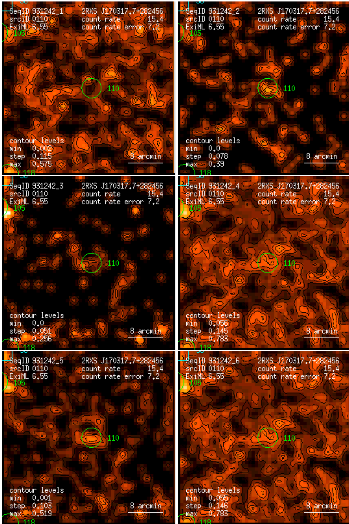
Figure 110: RASS 931242: detection 0110: band rate images, Gaussian filter: (1) PSPC channels 11 – 41, (2) 52 – 90, (3) 91 – 201, (4) 11 – 235, (5) 52 – 201, (6) 11 – 201. Broad band rates in counts/ks. Band rate contour levels in counts/ks/arcmin 2 .
