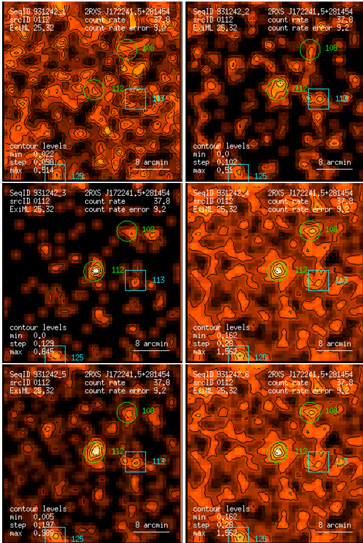
Figure 112: RASS 931242: detection 0112: band rate images, Gaussian filter: (1) PSPC channels 11 – 41, (2) 52 – 90, (3) 91 – 201, (4) 11 – 235, (5) 52 – 201, (6) 11 – 201. Broad band rates in counts/ks. Band rate contour levels in counts/ks/arcmin 2 .
