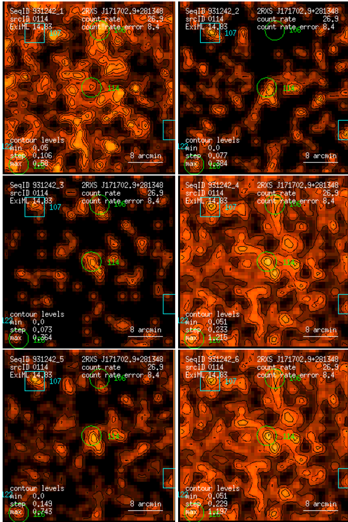
Figure 114: RASS 931242: detection 0114: band rate images, Gaussian filter: (1) PSPC channels 11 – 41, (2) 52 – 90, (3) 91 – 201, (4) 11 – 235, (5) 52 – 201, (6) 11 – 201. Broad band rates in counts/ks. Band rate contour levels in counts/ks/arcmin 2 .
