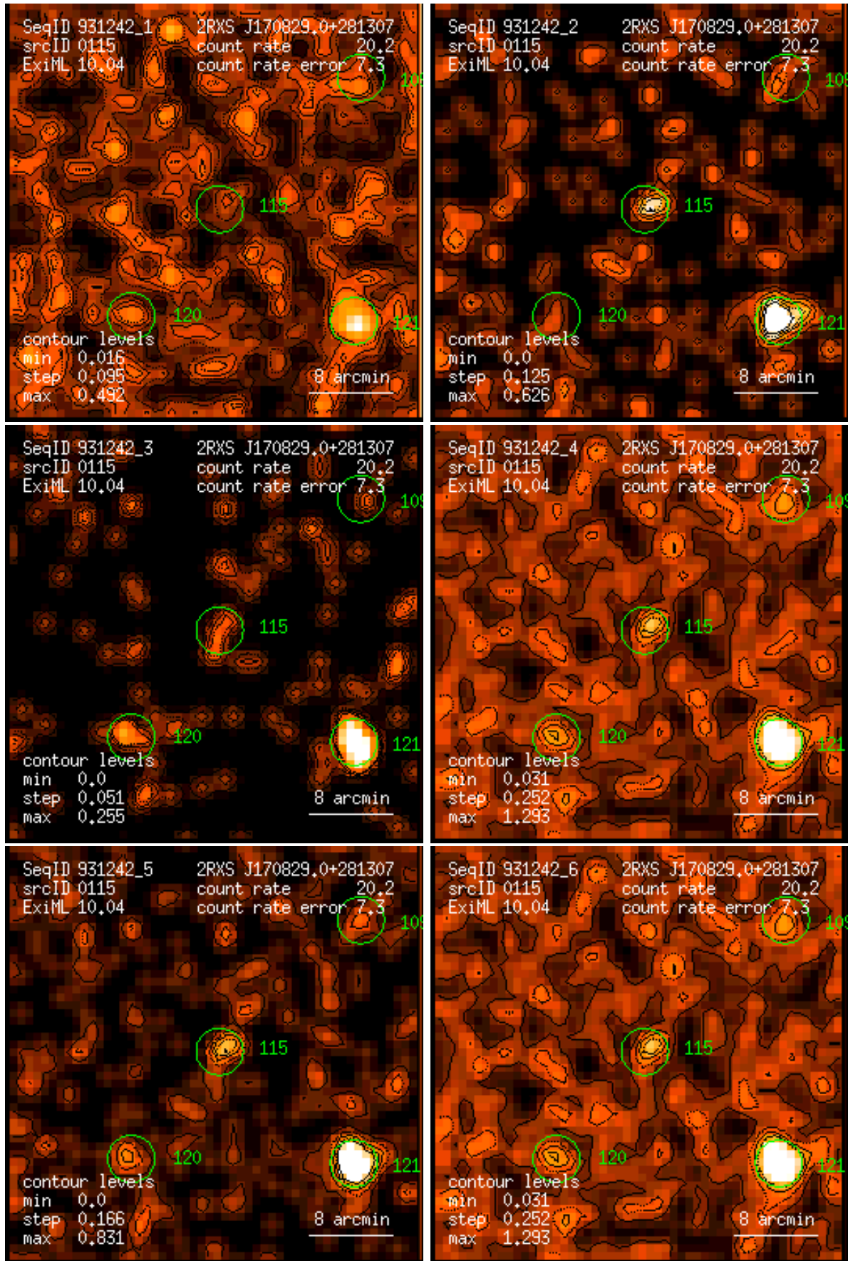
Figure 115: RASS 931242: detection 0115: band rate images, Gaussian filter: (1) PSPC channels 11 – 41, (2) 52 – 90, (3) 91 – 201, (4) 11 – 235, (5) 52 – 201, (6) 11 – 201. Broad band rates in counts/ks. Band rate contour levels in counts/ks/arcmin 2 .
