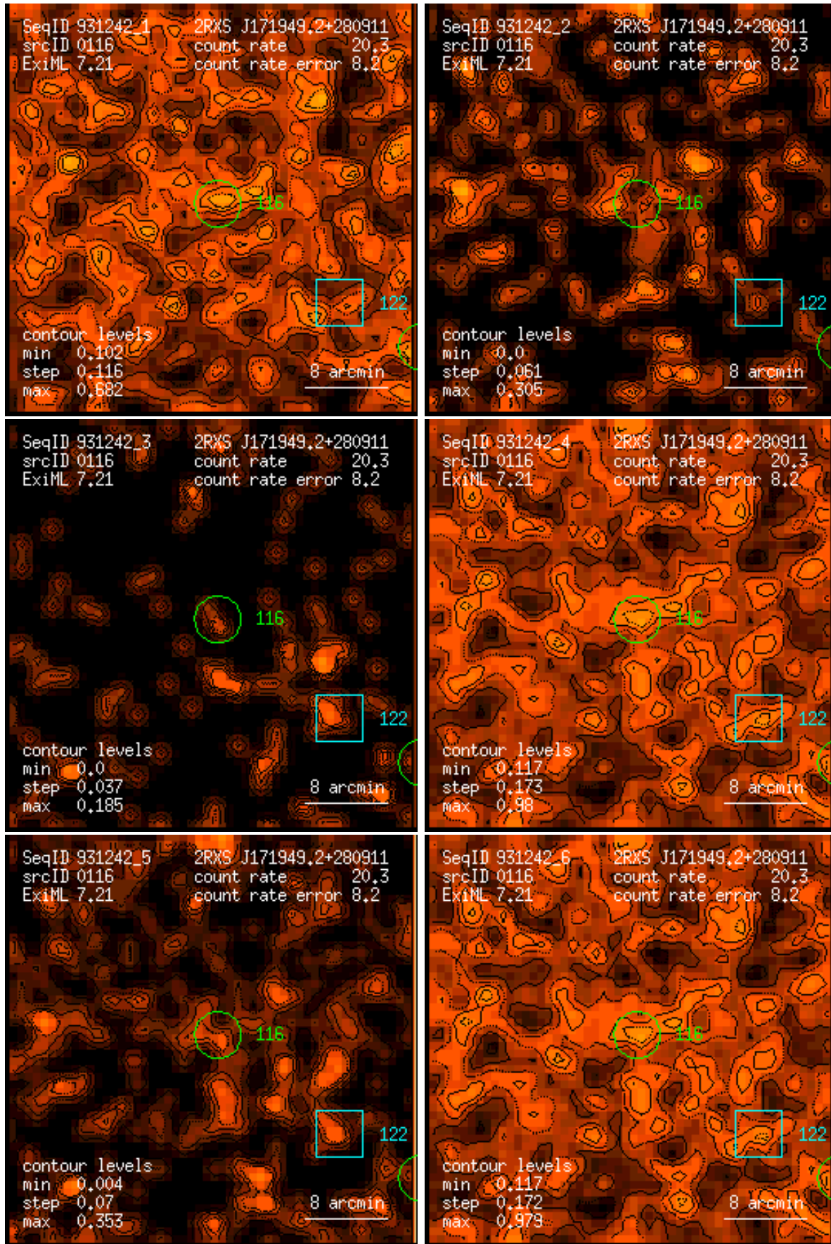
Figure 116: RASS 931242: detection 0116: band rate images, Gaussian filter: (1) PSPC channels 11 – 41, (2) 52 – 90, (3) 91 – 201, (4) 11 – 235, (5) 52 – 201, (6) 11 – 201. Broad band rates in counts/ks. Band rate contour levels in counts/ks/arcmin 2 .
