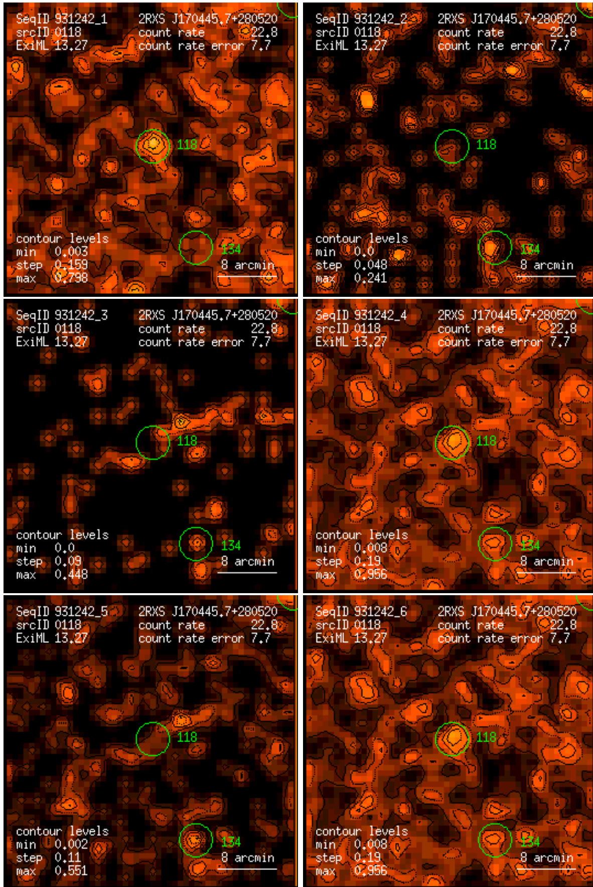
Figure 118: RASS 931242: detection 0118: band rate images, Gaussian filter: (1) PSPC channels 11 – 41, (2) 52 – 90, (3) 91 – 201, (4) 11 – 235, (5) 52 – 201, (6) 11 – 201. Broad band rates in counts/ks. Band rate contour levels in counts/ks/arcmin 2 .
