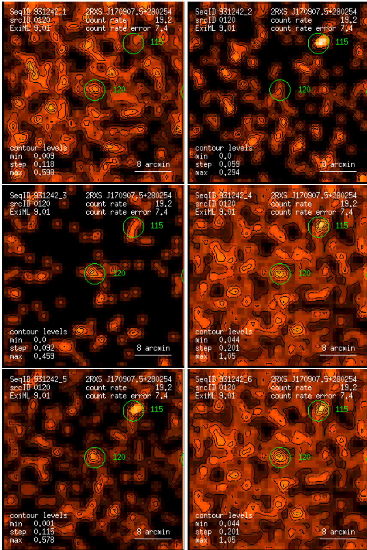
Figure 120: RASS 931242: detection 0120: band rate images, Gaussian filter: (1) PSPC channels 11 – 41, (2) 52 – 90, (3) 91 – 201, (4) 11 – 235, (5) 52 – 201, (6) 11 – 201. Broad band rates in counts/ks. Band rate contour levels in counts/ks/arcmin 2 .
