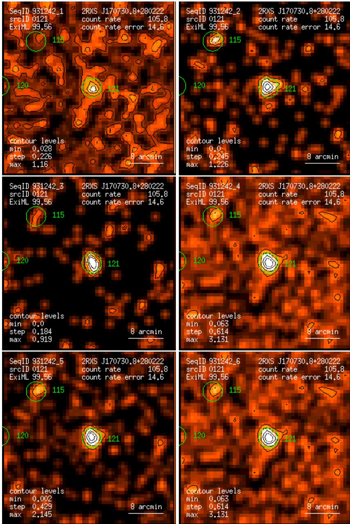
Figure 121: RASS 931242: detection 0121: band rate images, Gaussian filter: (1) PSPC channels 11 – 41, (2) 52 – 90, (3) 91 – 201, (4) 11 – 235, (5) 52 – 201, (6) 11 – 201. Broad band rates in counts/ks. Band rate contour levels in counts/ks/arcmin 2 .
