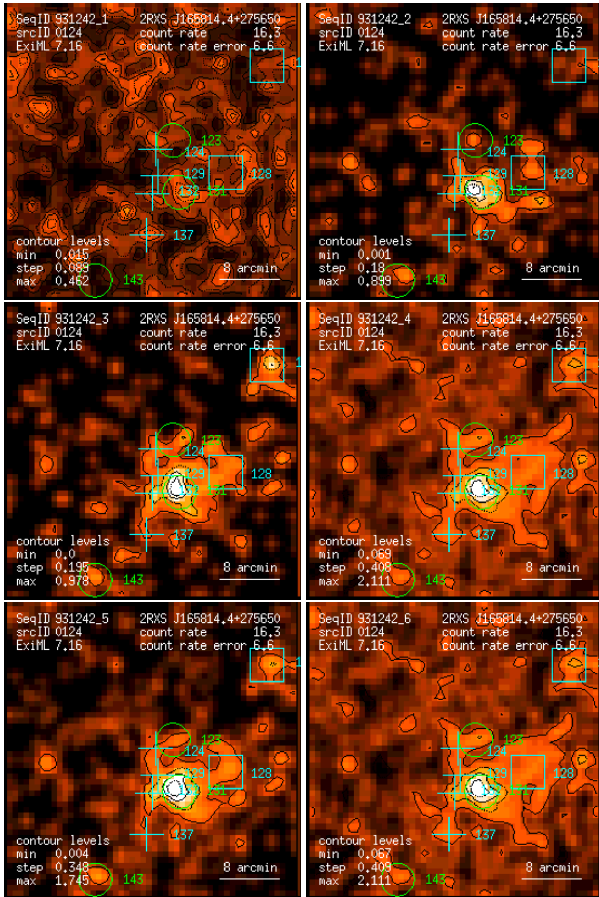
Figure 124: RASS 931242: detection 0124: band rate images, Gaussian filter: (1) PSPC channels 11 – 41, (2) 52 – 90, (3) 91 – 201, (4) 11 – 235, (5) 52 – 201, (6) 11 – 201. Broad band rates in counts/ks. Band rate contour levels in counts/ks/arcmin 2 .
