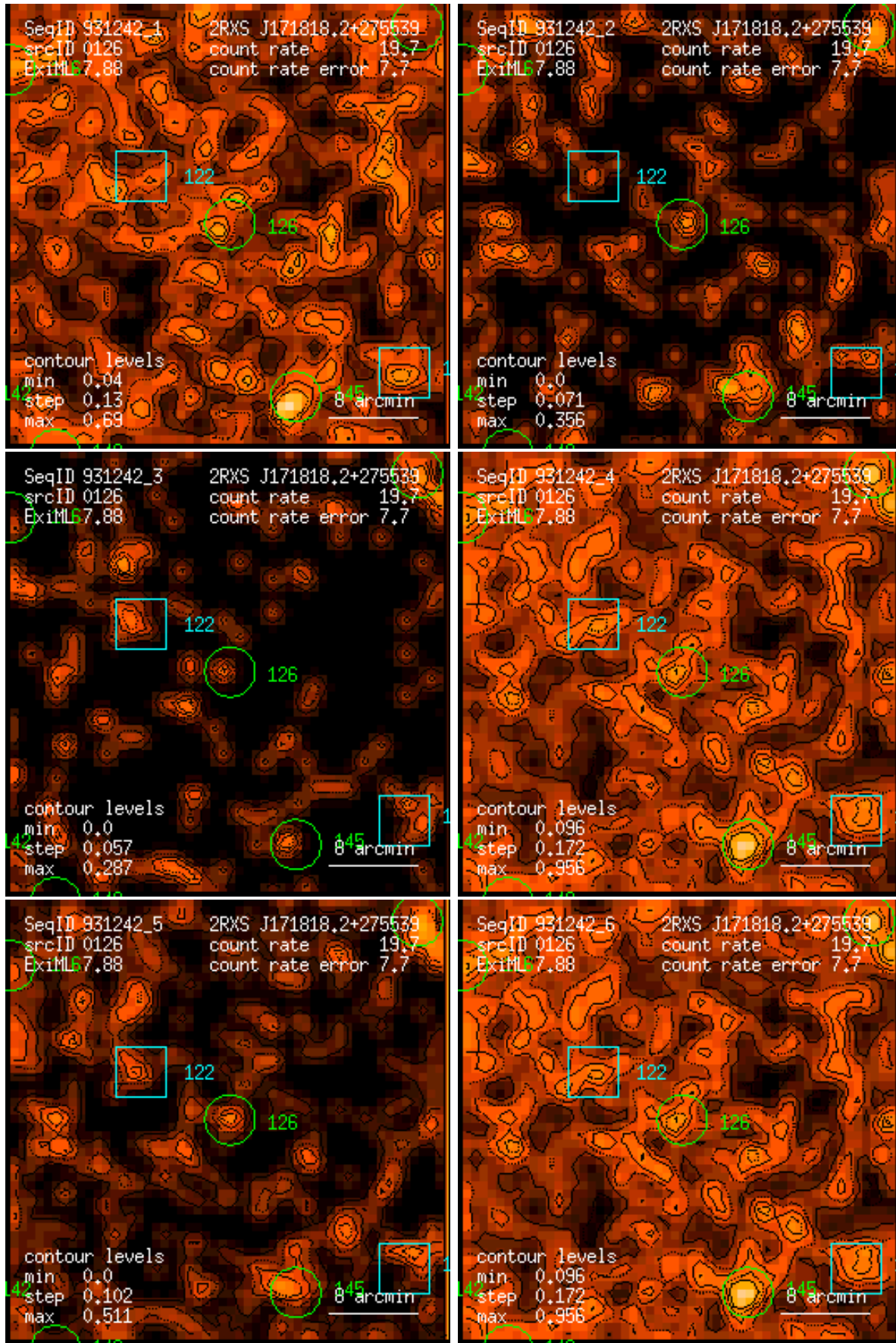
Figure 126: RASS 931242: detection 0126: band rate images, Gaussian filter: (1) PSPC channels 11 – 41, (2) 52 – 90, (3) 91 – 201, (4) 11 – 235, (5) 52 – 201, (6) 11 – 201. Broad band rates in counts/ks. Band rate contour levels in counts/ks/arcmin 2 .
