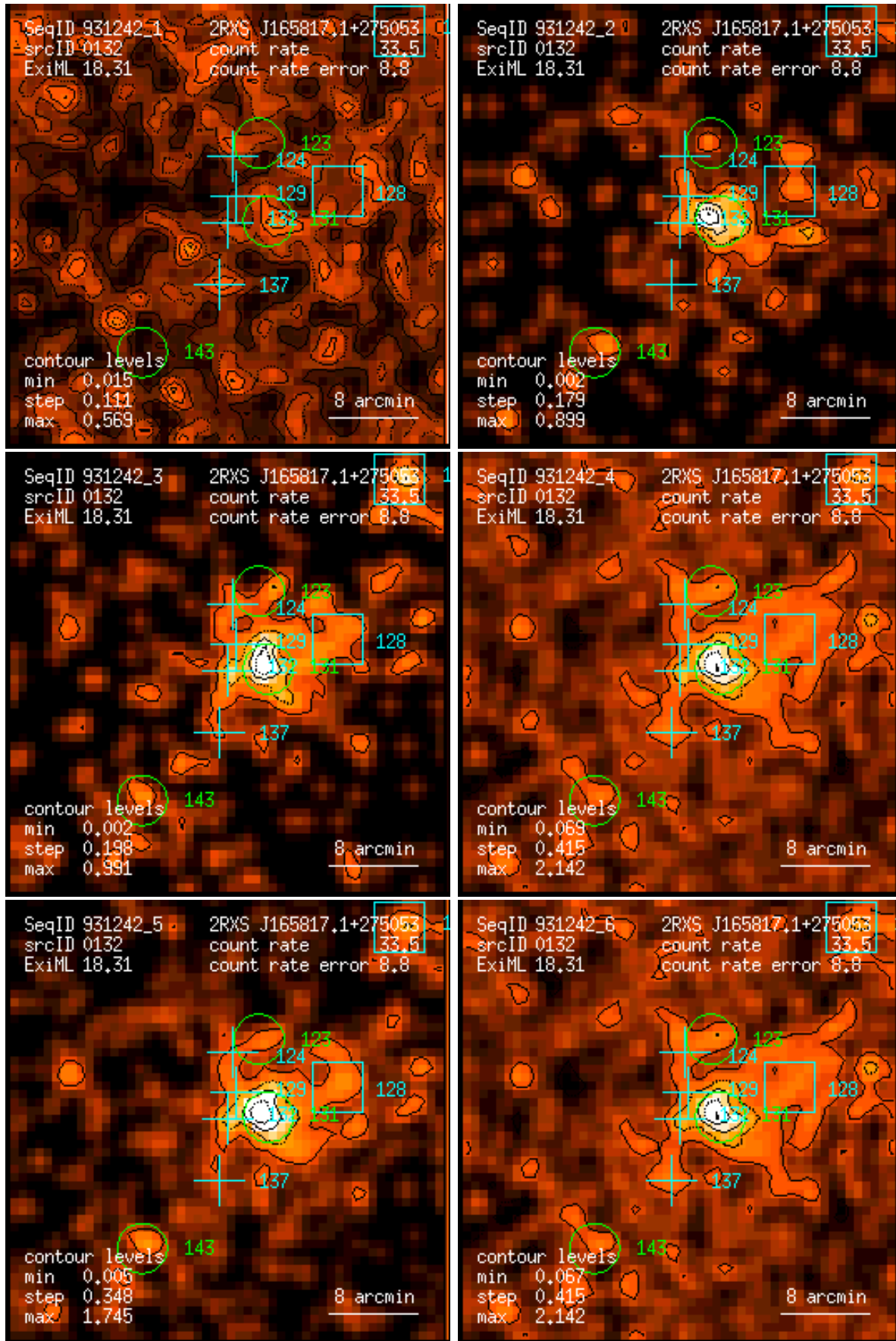
Figure 132: RASS 931242: detection 0132: band rate images, Gaussian filter: (1) PSPC channels 11 – 41, (2) 52 – 90, (3) 91 – 201, (4) 11 – 235, (5) 52 – 201, (6) 11 – 201. Broad band rates in counts/ks. Band rate contour levels in counts/ks/arcmin 2 .
