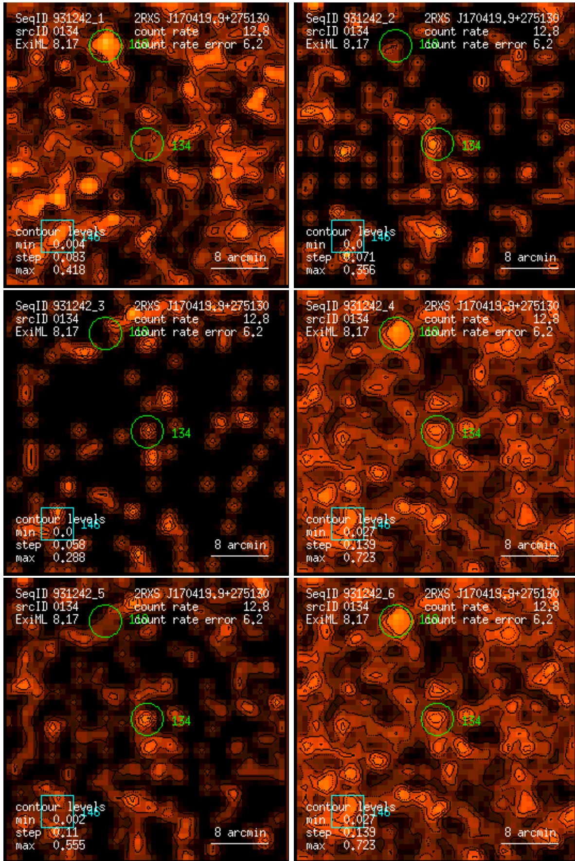
Figure 134: RASS 931242: detection 0134: band rate images, Gaussian filter: (1) PSPC channels 11 – 41, (2) 52 – 90, (3) 91 – 201, (4) 11 – 235, (5) 52 – 201, (6) 11 – 201. Broad band rates in counts/ks. Band rate contour levels in counts/ks/arcmin 2 .
