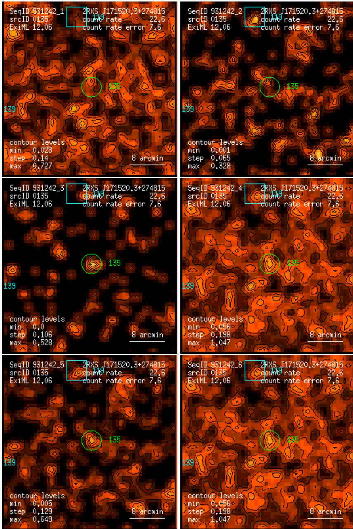
Figure 135: RASS 931242: detection 0135: band rate images, Gaussian filter: (1) PSPC channels 11 – 41, (2) 52 – 90, (3) 91 – 201, (4) 11 – 235, (5) 52 – 201, (6) 11 – 201. Broad band rates in counts/ks. Band rate contour levels in counts/ks/arcmin 2 .
