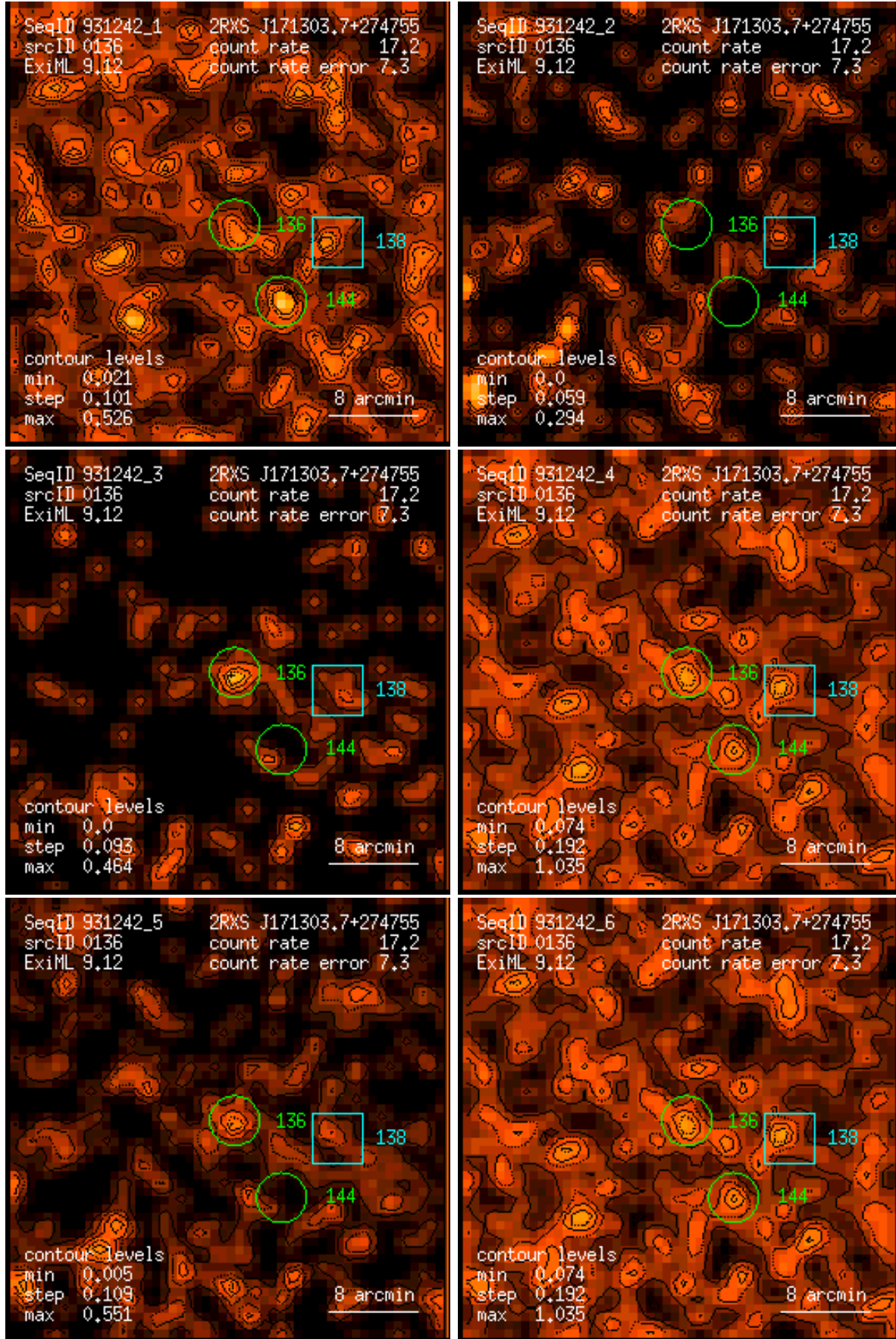
Figure 136: RASS 931242: detection 0136: band rate images, Gaussian filter: (1) PSPC channels 11 – 41, (2) 52 – 90, (3) 91 – 201, (4) 11 – 235, (5) 52 – 201, (6) 11 – 201. Broad band rates in counts/ks. Band rate contour levels in counts/ks/arcmin 2 .
