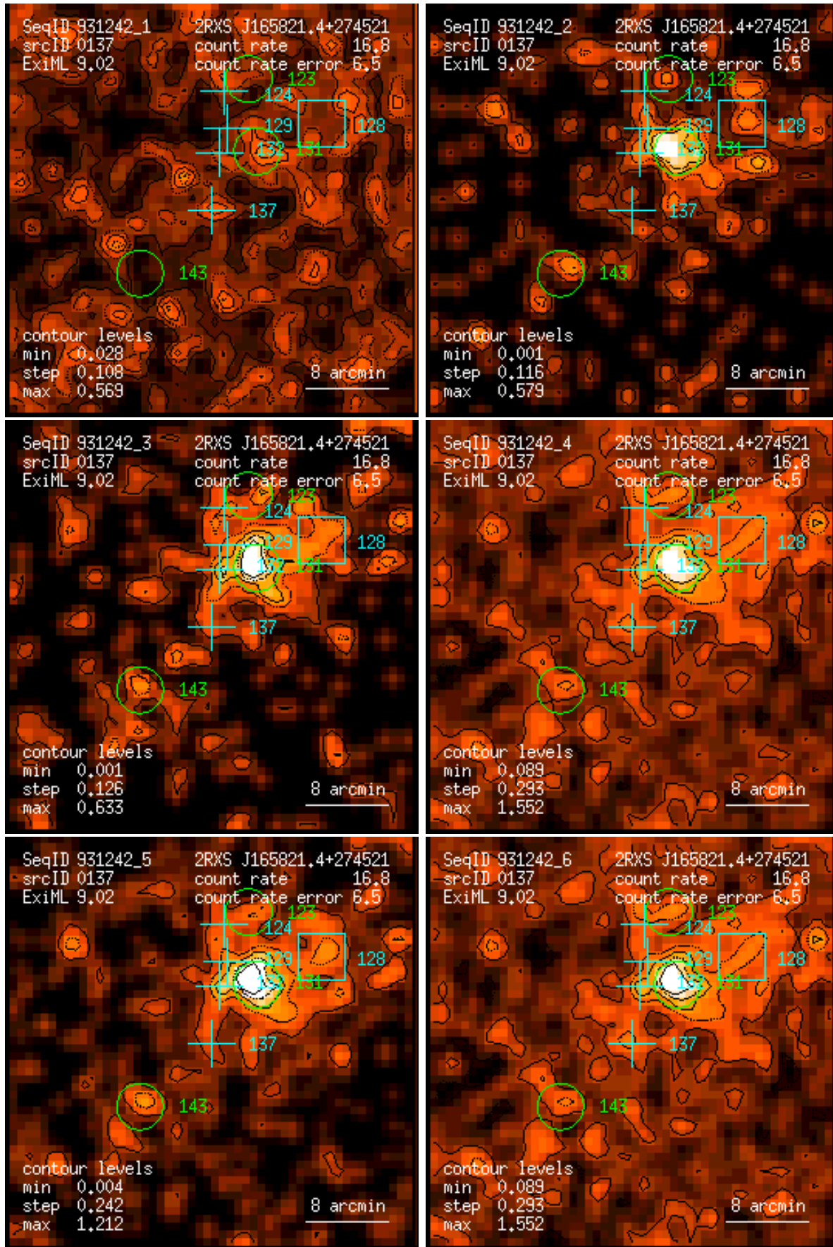
Figure 137: RASS 931242: detection 0137: band rate images, Gaussian filter: (1) PSPC channels 11 – 41, (2) 52 – 90, (3) 91 – 201, (4) 11 – 235, (5) 52 – 201, (6) 11 – 201. Broad band rates in counts/ks. Band rate contour levels in counts/ks/arcmin 2 .
