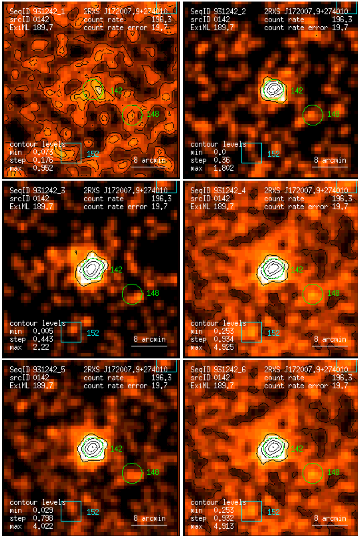
Figure 142: RASS 931242: detection 0142: band rate images, Gaussian filter: (1) PSPC channels 11 – 41, (2) 52 – 90, (3) 91 – 201, (4) 11 – 235, (5) 52 – 201, (6) 11 – 201. Broad band rates in counts/ks. Band rate contour levels in counts/ks/arcmin 2 .
