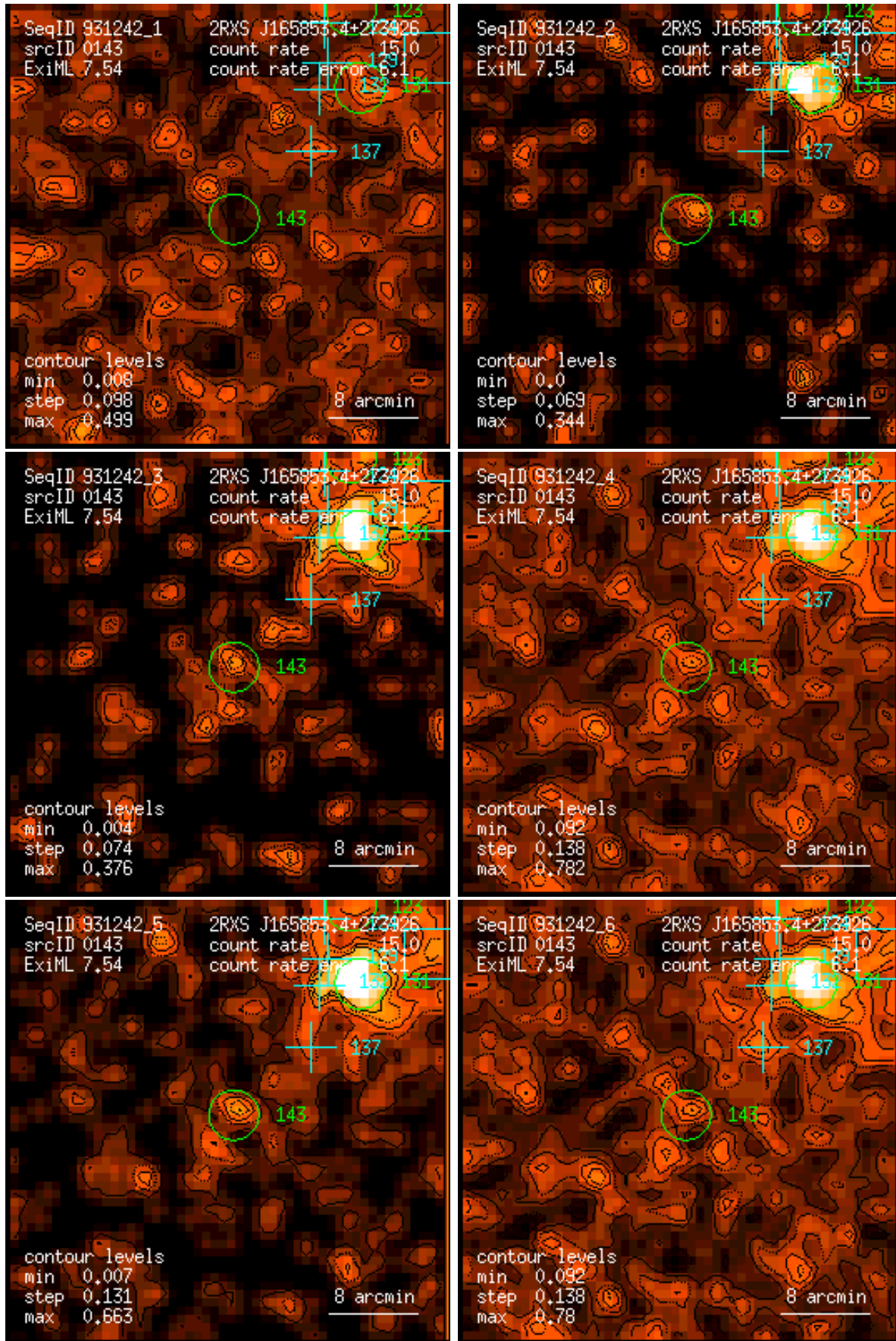
Figure 143: RASS 931242: detection 0143: band rate images, Gaussian filter: (1) PSPC channels 11 – 41, (2) 52 – 90, (3) 91 – 201, (4) 11 – 235, (5) 52 – 201, (6) 11 – 201. Broad band rates in counts/ks. Band rate contour levels in counts/ks/arcmin 2 .
