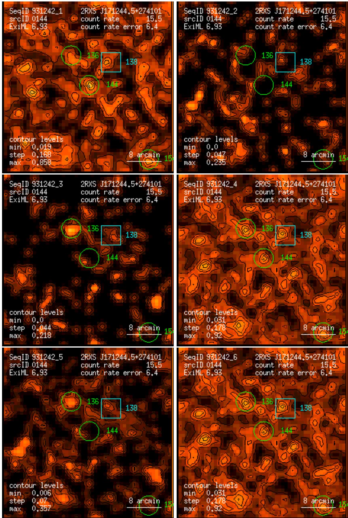
Figure 144: RASS 931242: detection 0144: band rate images, Gaussian filter: (1) PSPC channels 11 – 41, (2) 52 – 90, (3) 91 – 201, (4) 11 – 235, (5) 52 – 201, (6) 11 – 201. Broad band rates in counts/ks. Band rate contour levels in counts/ks/arcmin 2 .
