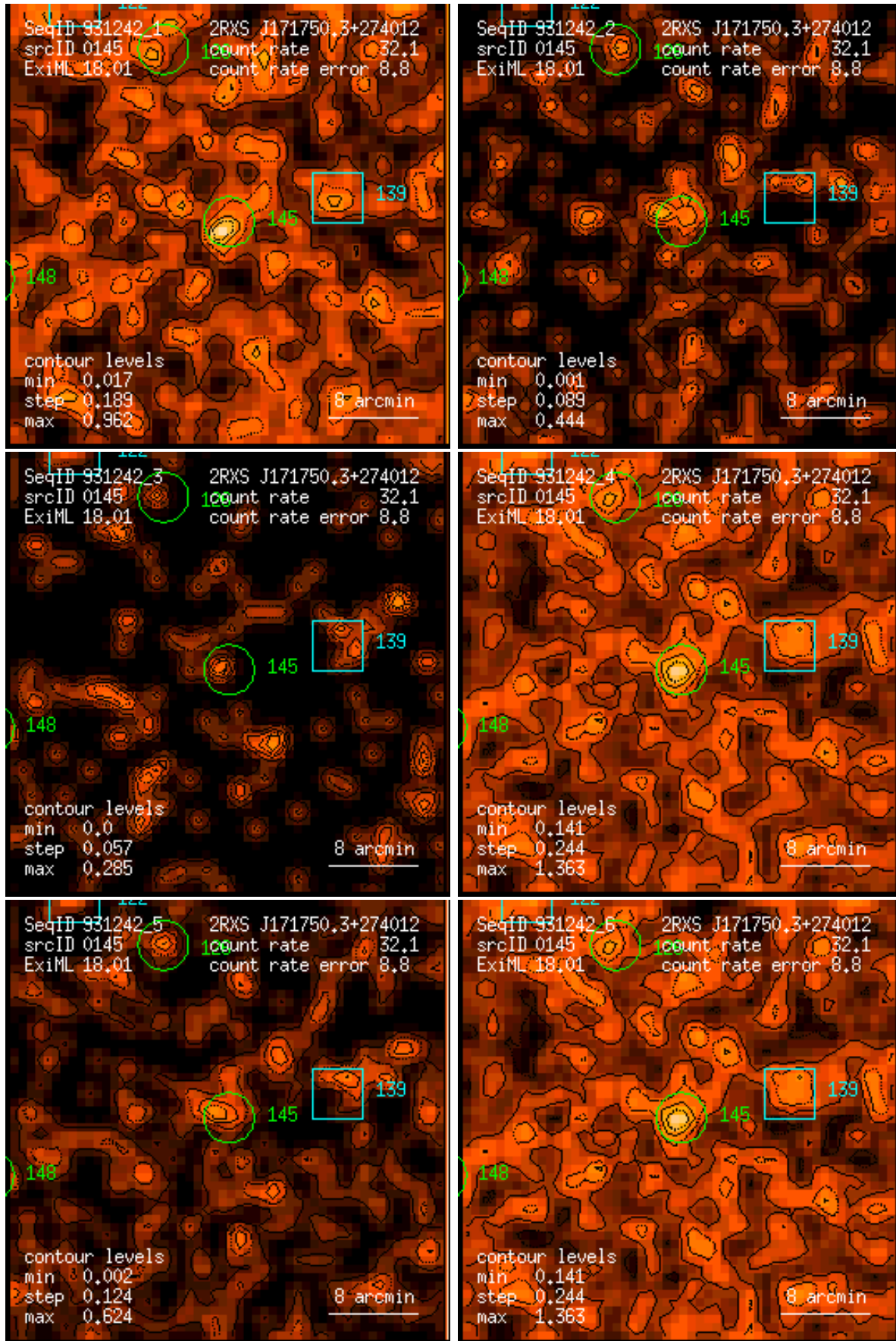
Figure 145: RASS 931242: detection 0145: band rate images, Gaussian filter: (1) PSPC channels 11 – 41, (2) 52 – 90, (3) 91 – 201, (4) 11 – 235, (5) 52 – 201, (6) 11 – 201. Broad band rates in counts/ks. Band rate contour levels in counts/ks/arcmin 2 .
