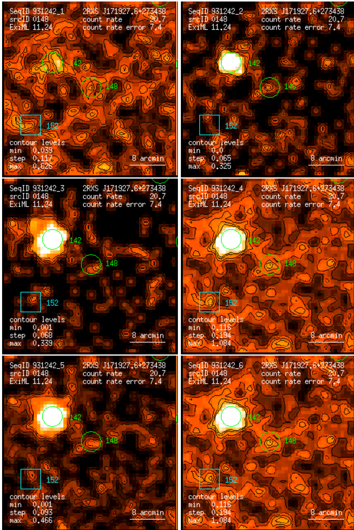
Figure 148: RASS 931242: detection 0148: band rate images, Gaussian filter: (1) PSPC channels 11 – 41, (2) 52 – 90, (3) 91 – 201, (4) 11 – 235, (5) 52 – 201, (6) 11 – 201. Broad band rates in counts/ks. Band rate contour levels in counts/ks/arcmin 2 .
