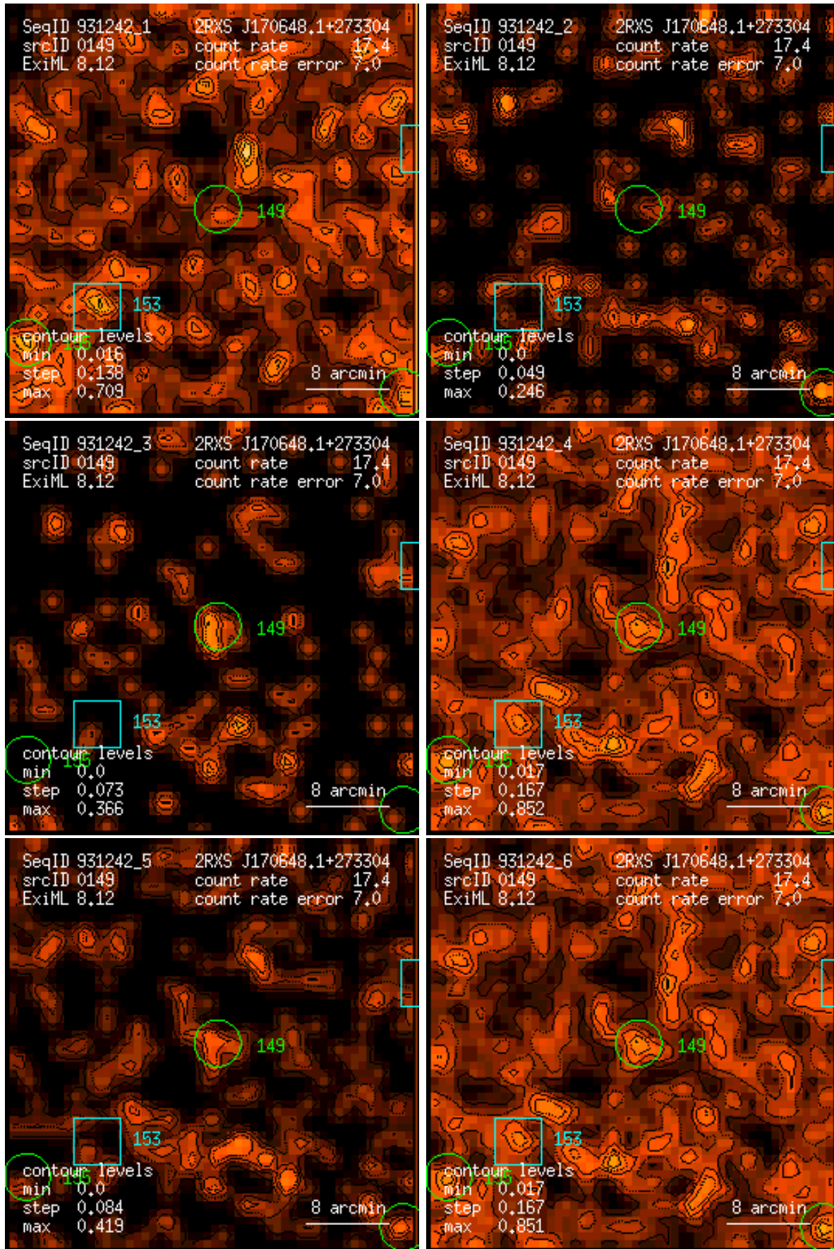
Figure 149: RASS 931242: detection 0149: band rate images, Gaussian filter: (1) PSPC channels 11 – 41, (2) 52 – 90, (3) 91 – 201, (4) 11 – 235, (5) 52 – 201, (6) 11 – 201. Broad band rates in counts/ks. Band rate contour levels in counts/ks/arcmin 2 .
