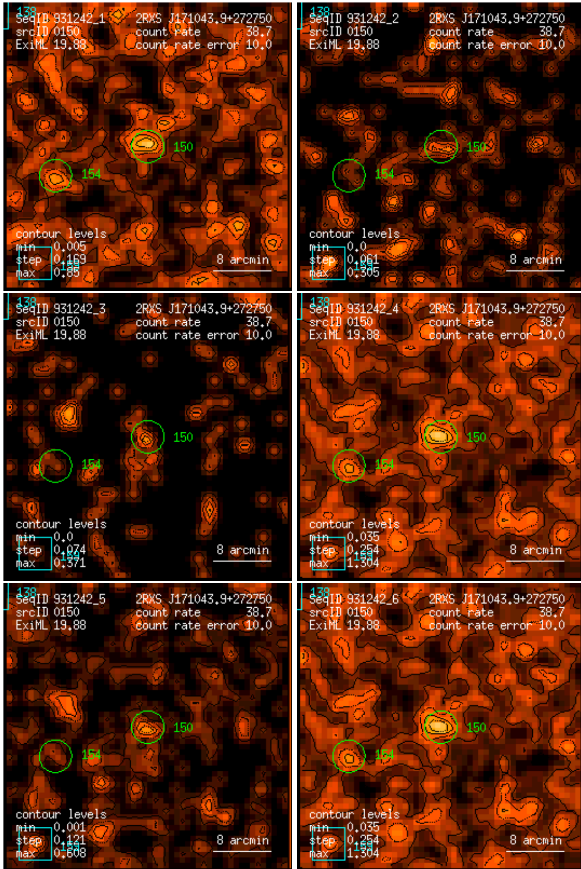
Figure 150: RASS 931242: detection 0150: band rate images, Gaussian filter: (1) PSPC channels 11 – 41, (2) 52 – 90, (3) 91 – 201, (4) 11 – 235, (5) 52 – 201, (6) 11 – 201. Broad band rates in counts/ks. Band rate contour levels in counts/ks/arcmin 2 .
