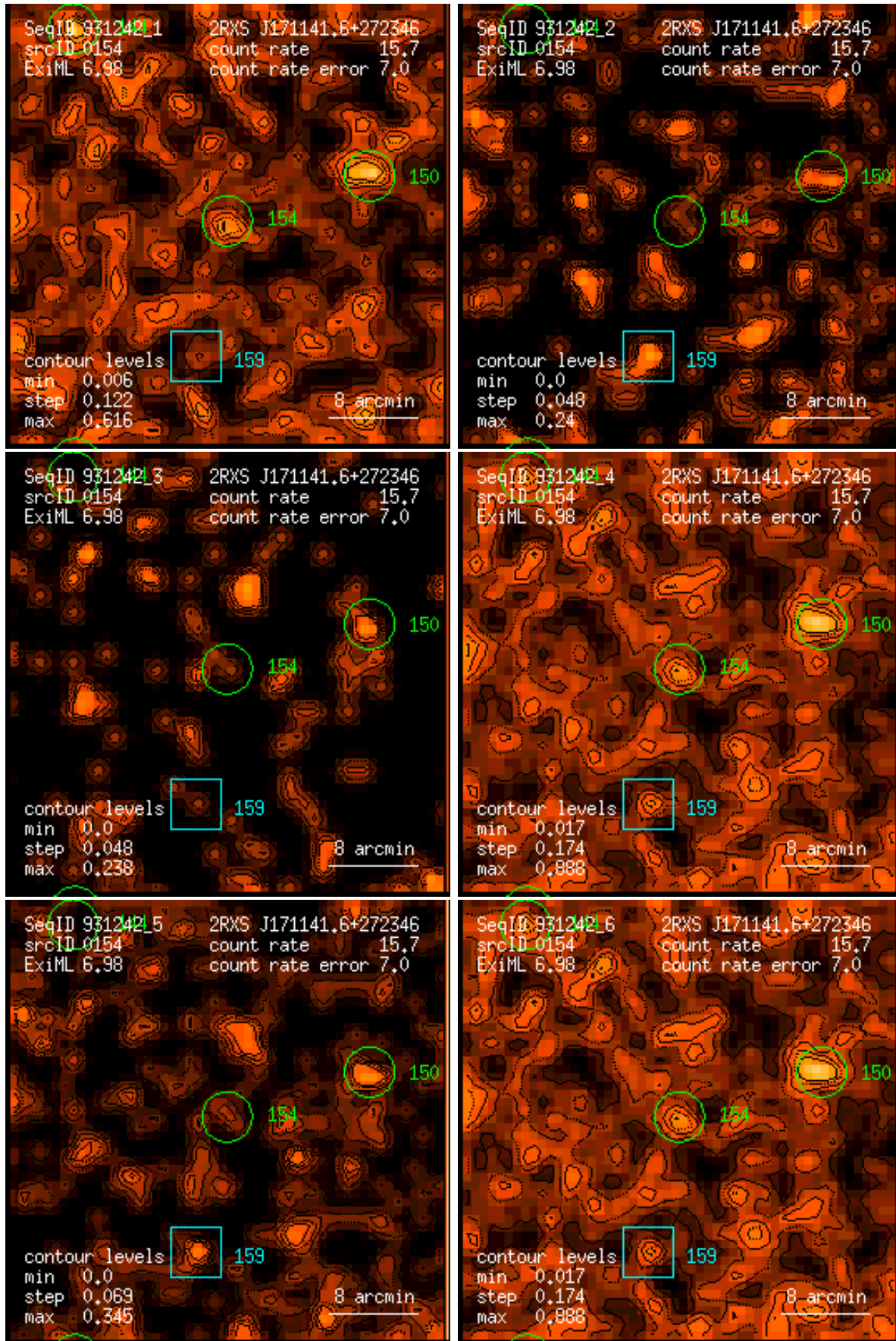
Figure 154: RASS 931242: detection 0154: band rate images, Gaussian filter: (1) PSPC channels 11 – 41, (2) 52 – 90, (3) 91 – 201, (4) 11 – 235, (5) 52 – 201, (6) 11 – 201. Broad band rates in counts/ks. Band rate contour levels in counts/ks/arcmin 2 .
