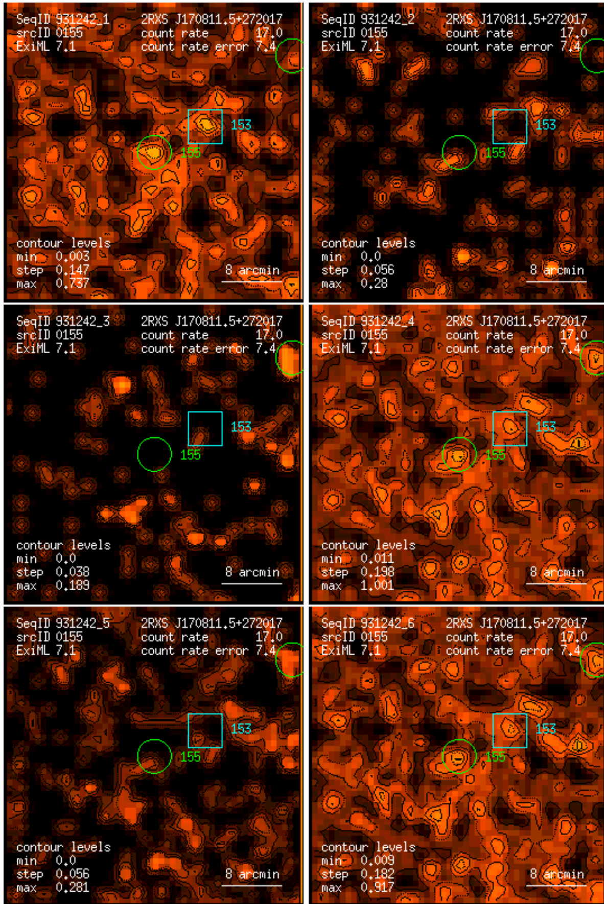
Figure 155: RASS 931242: detection 0155: band rate images, Gaussian filter: (1) PSPC channels 11 – 41, (2) 52 – 90, (3) 91 – 201, (4) 11 – 235, (5) 52 – 201, (6) 11 – 201. Broad band rates in counts/ks. Band rate contour levels in counts/ks/arcmin 2 .
