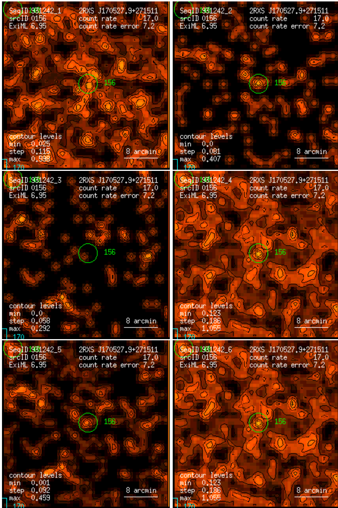
Figure 156: RASS 931242: detection 0156: band rate images, Gaussian filter: (1) PSPC channels 11 – 41, (2) 52 – 90, (3) 91 – 201, (4) 11 – 235, (5) 52 – 201, (6) 11 – 201. Broad band rates in counts/ks. Band rate contour levels in counts/ks/arcmin 2 .
