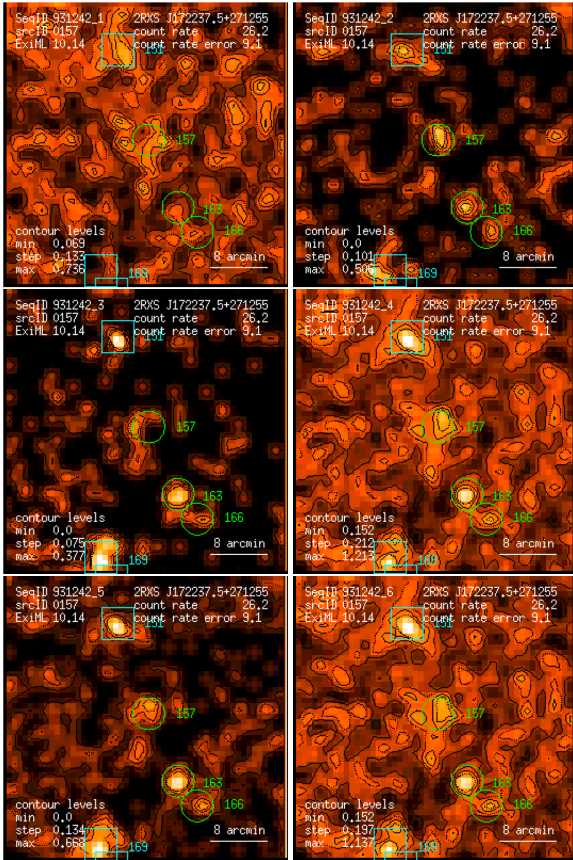
Figure 157: RASS 931242: detection 0157: band rate images, Gaussian filter: (1) PSPC channels 11 – 41, (2) 52 – 90, (3) 91 – 201, (4) 11 – 235, (5) 52 – 201, (6) 11 – 201. Broad band rates in counts/ks. Band rate contour levels in counts/ks/arcmin 2 .
