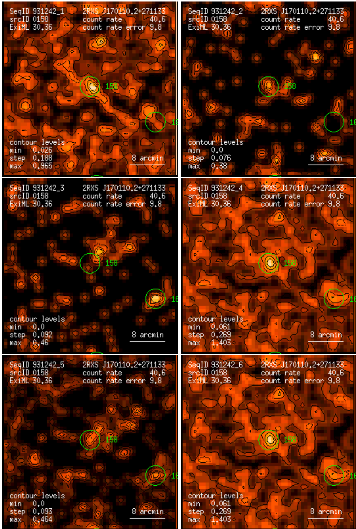
Figure 158: RASS 931242: detection 0158: band rate images, Gaussian filter: (1) PSPC channels 11 – 41, (2) 52 – 90, (3) 91 – 201, (4) 11 – 235, (5) 52 – 201, (6) 11 – 201. Broad band rates in counts/ks. Band rate contour levels in counts/ks/arcmin 2 .
