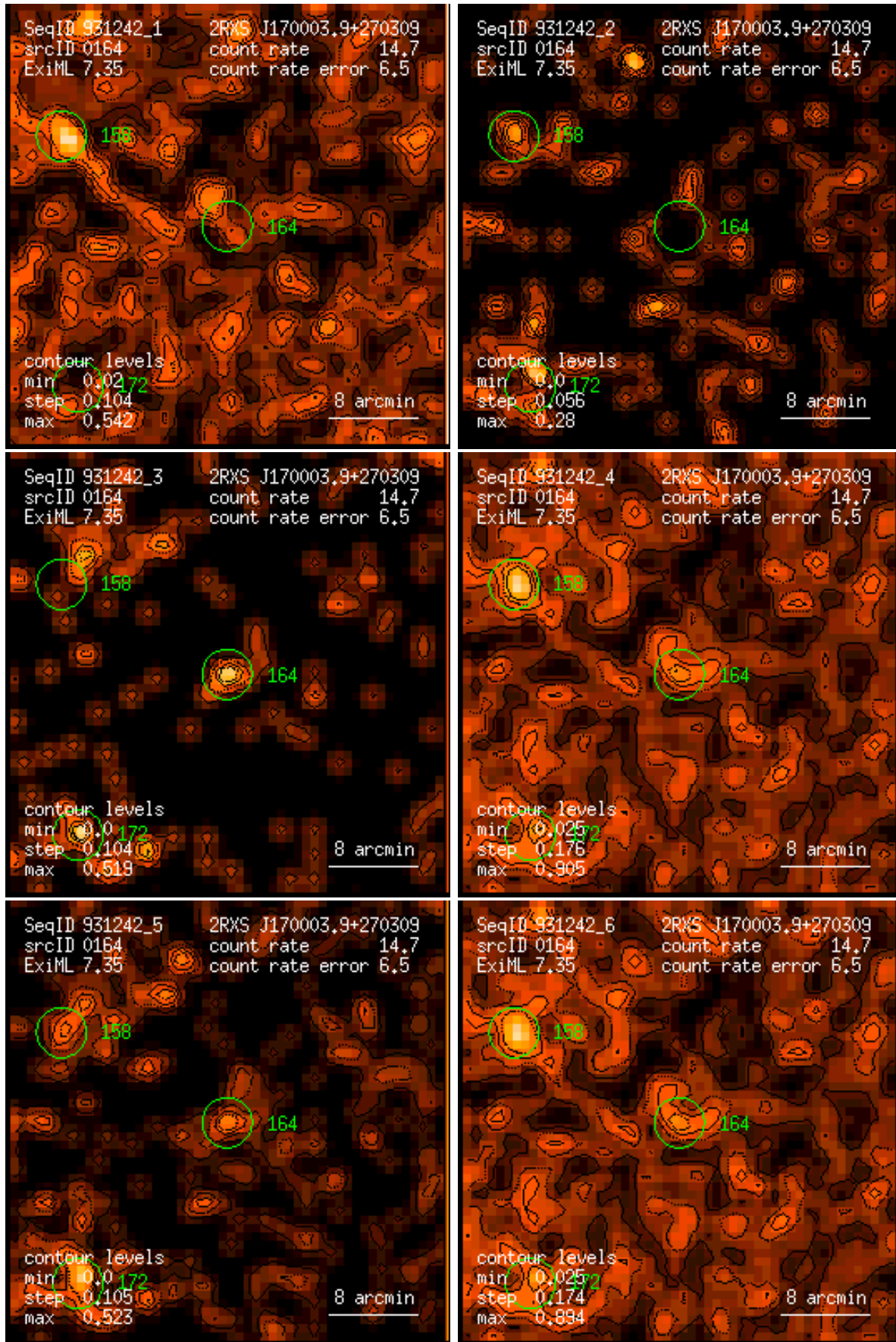
Figure 164: RASS 931242: detection 0164: band rate images, Gaussian filter: (1) PSPC channels 11 – 41, (2) 52 – 90, (3) 91 – 201, (4) 11 – 235, (5) 52 – 201, (6) 11 – 201. Broad band rates in counts/ks. Band rate contour levels in counts/ks/arcmin 2 .
