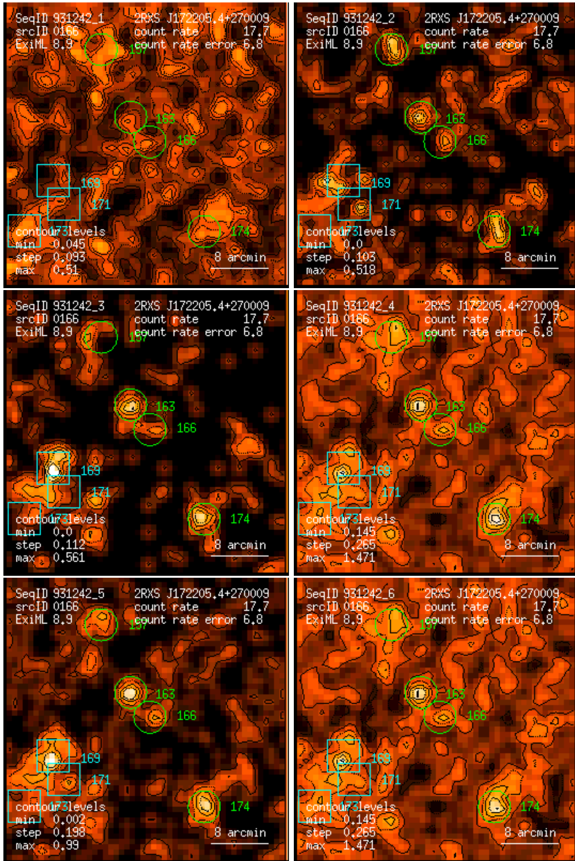
Figure 166: RASS 931242: detection 0166: band rate images, Gaussian filter: (1) PSPC channels 11 – 41, (2) 52 – 90, (3) 91 – 201, (4) 11 – 235, (5) 52 – 201, (6) 11 – 201. Broad band rates in counts/ks. Band rate contour levels in counts/ks/arcmin 2 .
