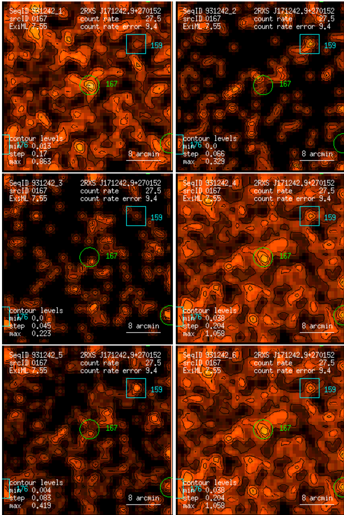
Figure 167: RASS 931242: detection 0167: band rate images, Gaussian filter: (1) PSPC channels 11 – 41, (2) 52 – 90, (3) 91 – 201, (4) 11 – 235, (5) 52 – 201, (6) 11 – 201. Broad band rates in counts/ks. Band rate contour levels in counts/ks/arcmin 2 .
