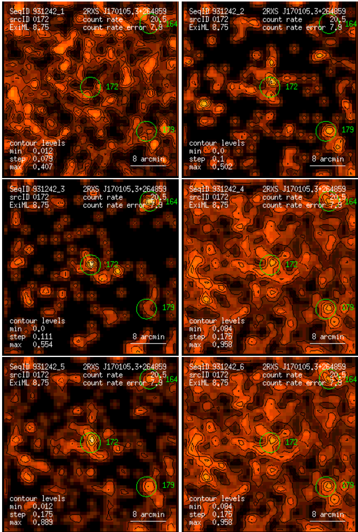
Figure 172: RASS 931242: detection 0172: band rate images, Gaussian filter: (1) PSPC channels 11 – 41, (2) 52 – 90, (3) 91 – 201, (4) 11 – 235, (5) 52 – 201, (6) 11 – 201. Broad band rates in counts/ks. Band rate contour levels in counts/ks/arcmin 2 .
