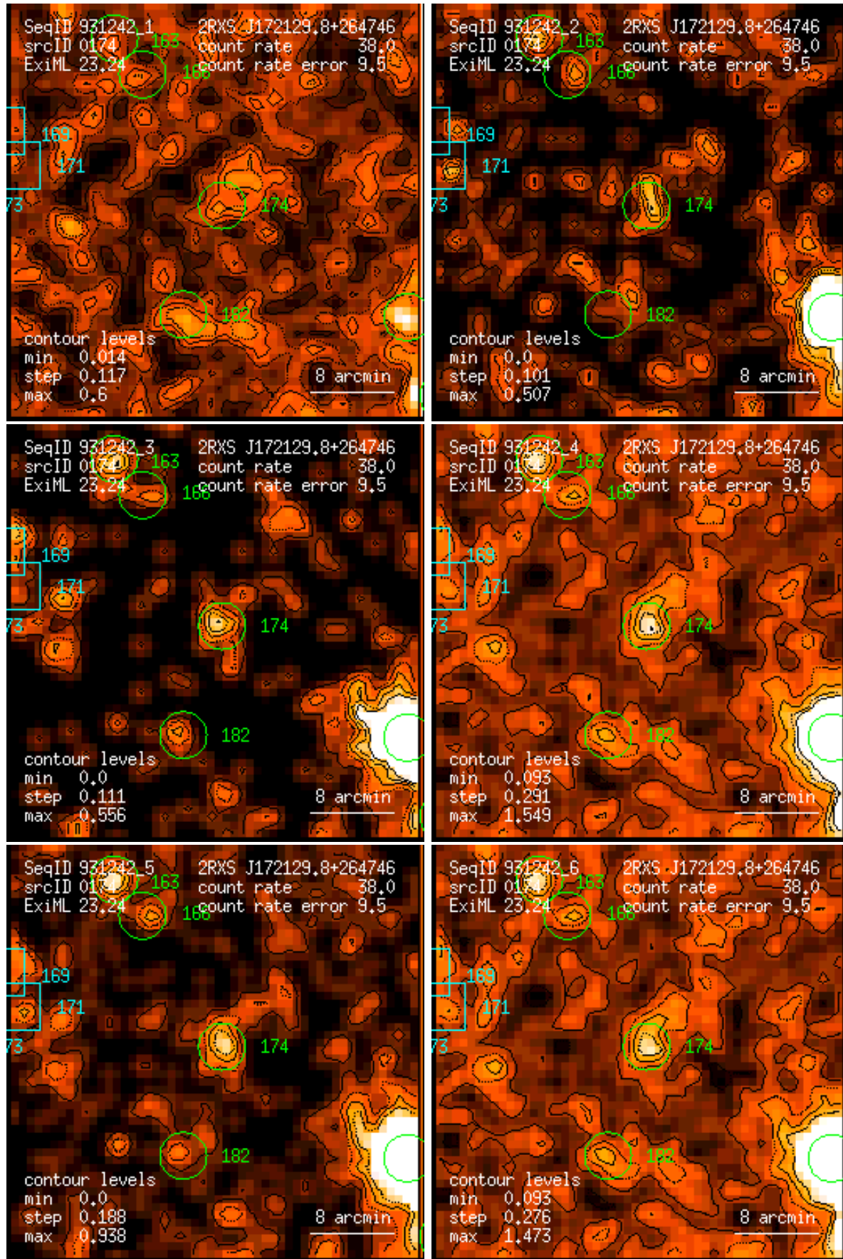
Figure 174: RASS 931242: detection 0174: band rate images, Gaussian filter: (1) PSPC channels 11 – 41, (2) 52 – 90, (3) 91 – 201, (4) 11 – 235, (5) 52 – 201, (6) 11 – 201. Broad band rates in counts/ks. Band rate contour levels in counts/ks/arcmin 2 .
